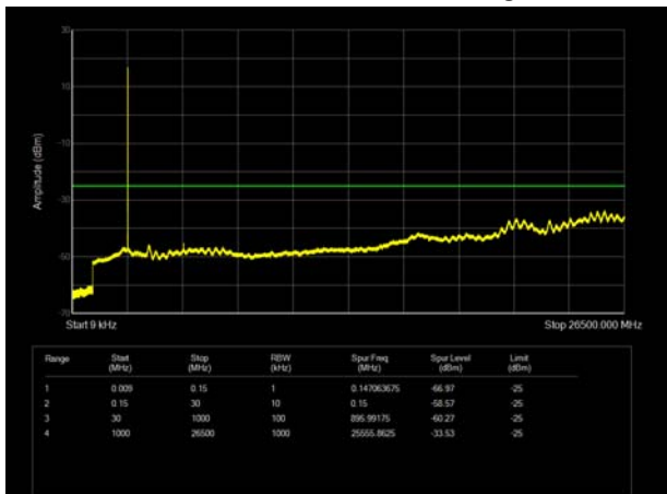
LTE Band 41 5MHz CH-High
