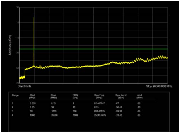
LTE Band 41 5MHz CH-Middle
