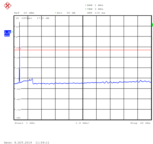
LTE Band 4 1.4MHz CH-High 1GHz~20GHz
