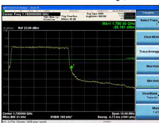
LTE Band 66 16QAM 5MHz CH-High, 100%RB
