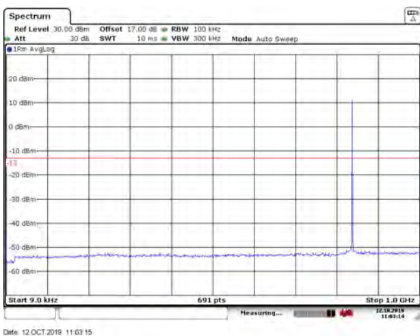
LTE Band 5 1.4MHz CH-Middle 9kHz~1GHz
