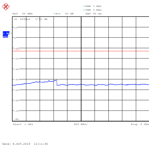
LTE Band 5 1.4MHz CH-High 1GHz~9GHz
