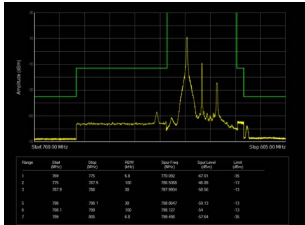
LTE Band 14 64QAM 5MHz 100%RB CH-23255
