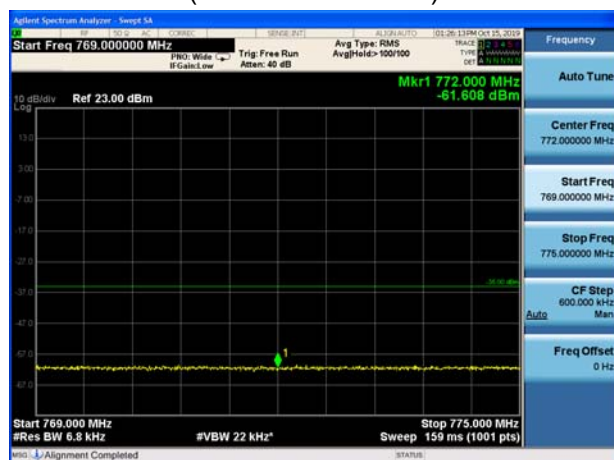
LTE Band 14 QPSK 5MHz 1 RB CH-Low (769MHz ~775MHz)
