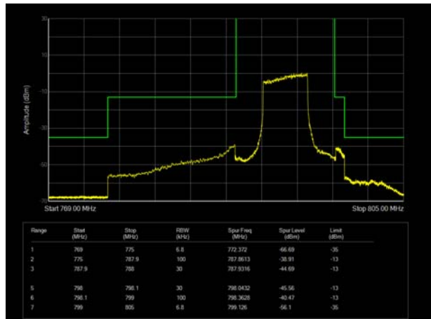
LTE Band 14 64QAM 10MHz 100%RB CH-23230
