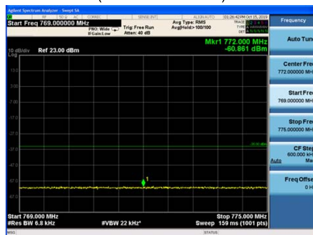
LTE Band 14 QPSK 5MHz 100%RB CH-Low (769MHz ~775MHz)
