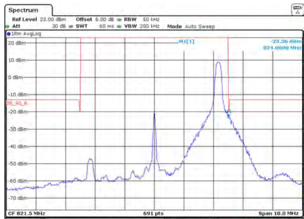
LTE Band 26 16QAM 5MHz CH-High 1RB
