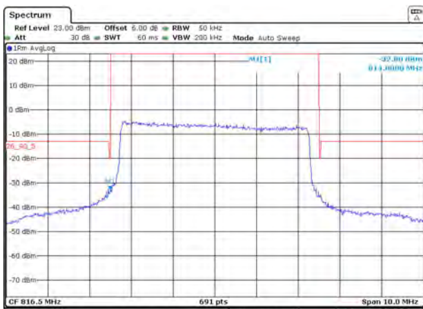
LTE Band 26 16QAM 5MHz CH-Low 100%RB
