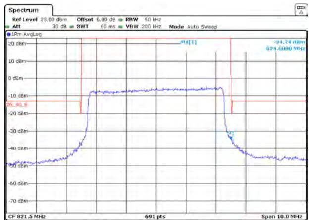
LTE Band 26 QPSK 5MHz CH-High 100%RB
