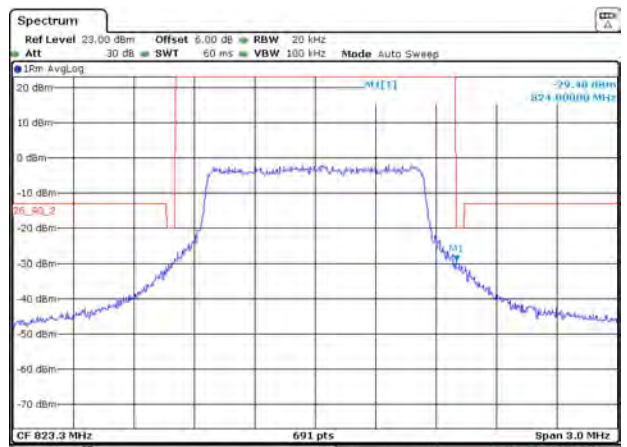
LTE Band 26 16QAM 1.4MHz CH-High 100%RB
