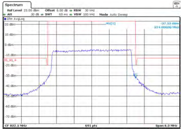
LTE Band 26 QPSK 3MHz CH-High 100%RB
