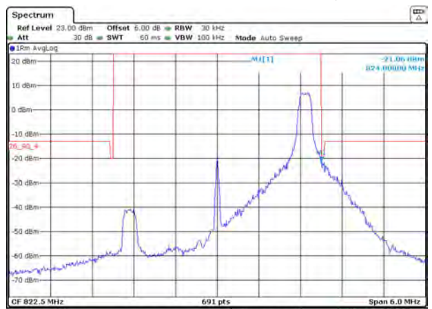
LTE Band 26 16QAM 3MHz CH-High 1RB
