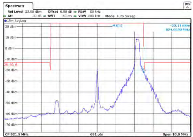
LTE Band 26 QPSK 5MHz CH-High 1RB
