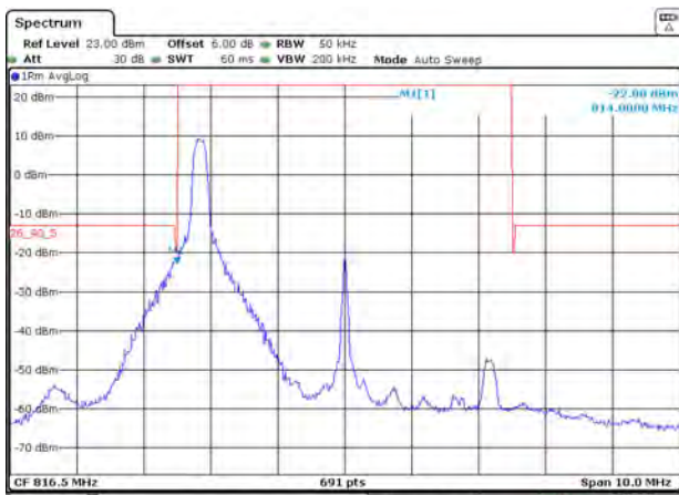
LTE Band 26 16QAM 5MHz CH-Low 1RB
