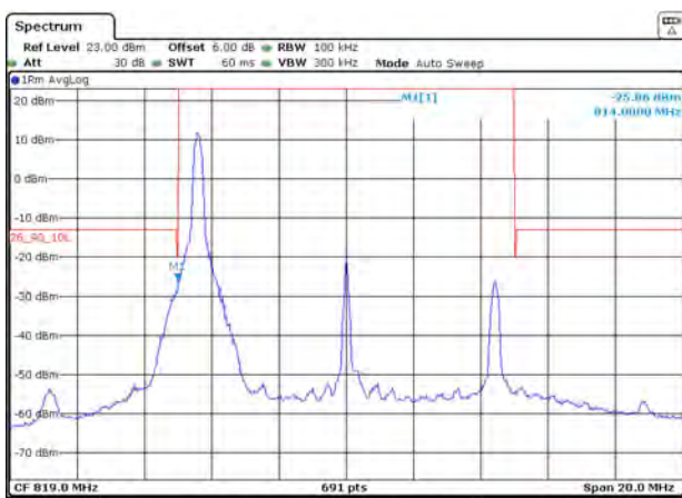
LTE Band 26 16QAM 10MHz CH-Low 1RB
