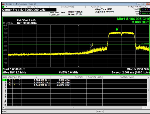
(802.1n40) Band Edge, Left Side
