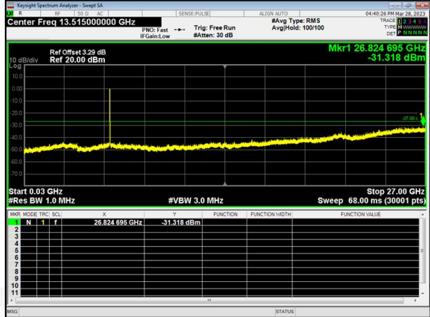
802.11n20 on channel 159
