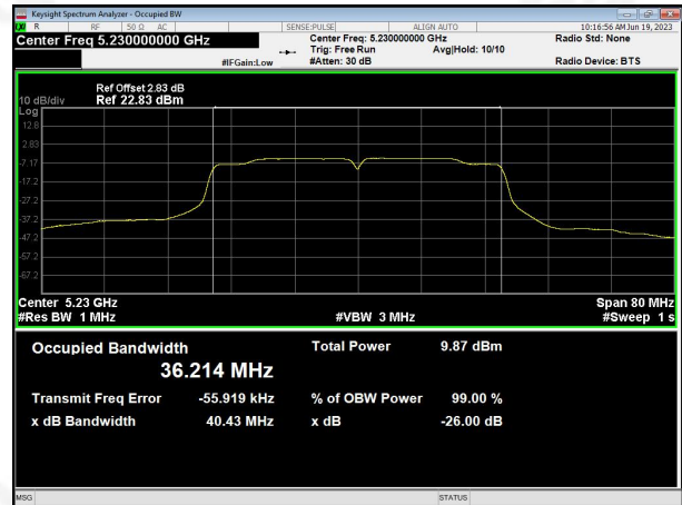
(802.11 n40) 26dB Bandwidth plot on channel 46
