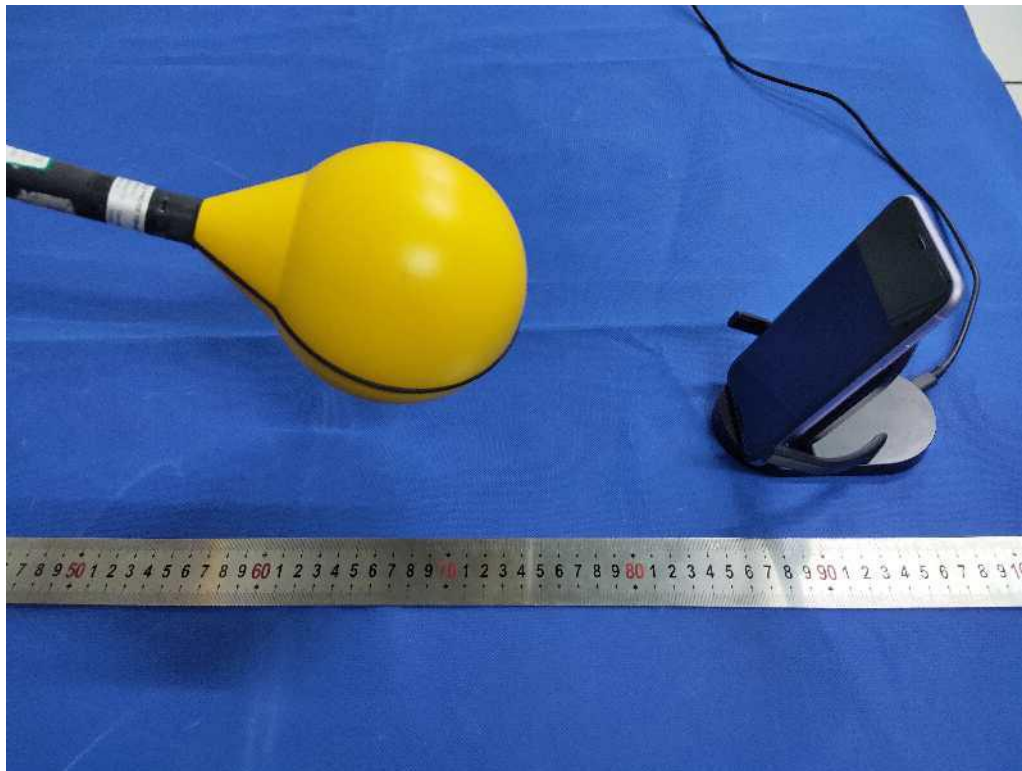
Magnetic Field Emissions Test Photo
