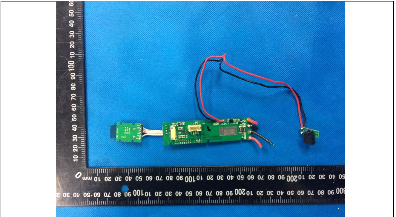
Details of: PCB view for main board
