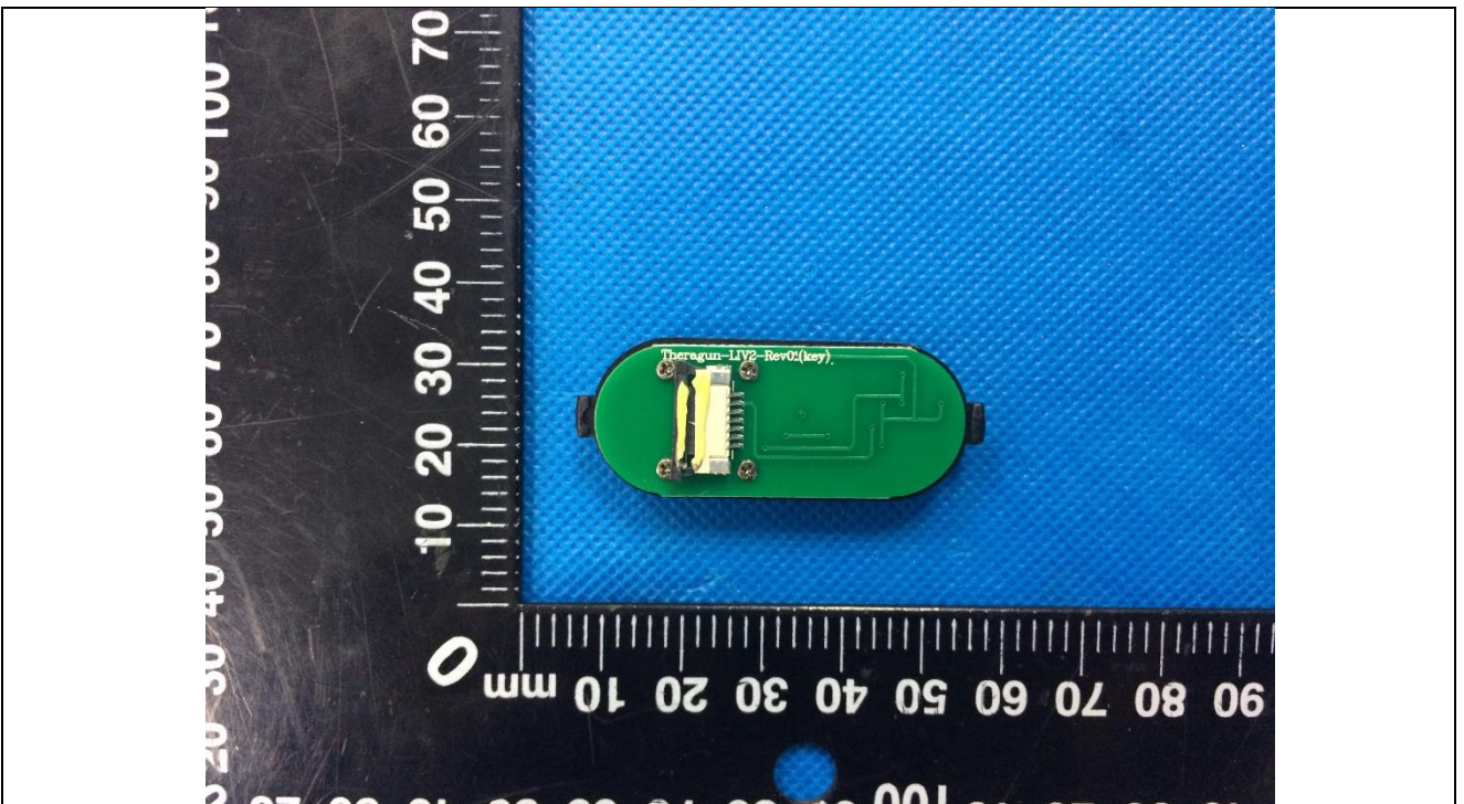
Details of: PCB view for Button board
