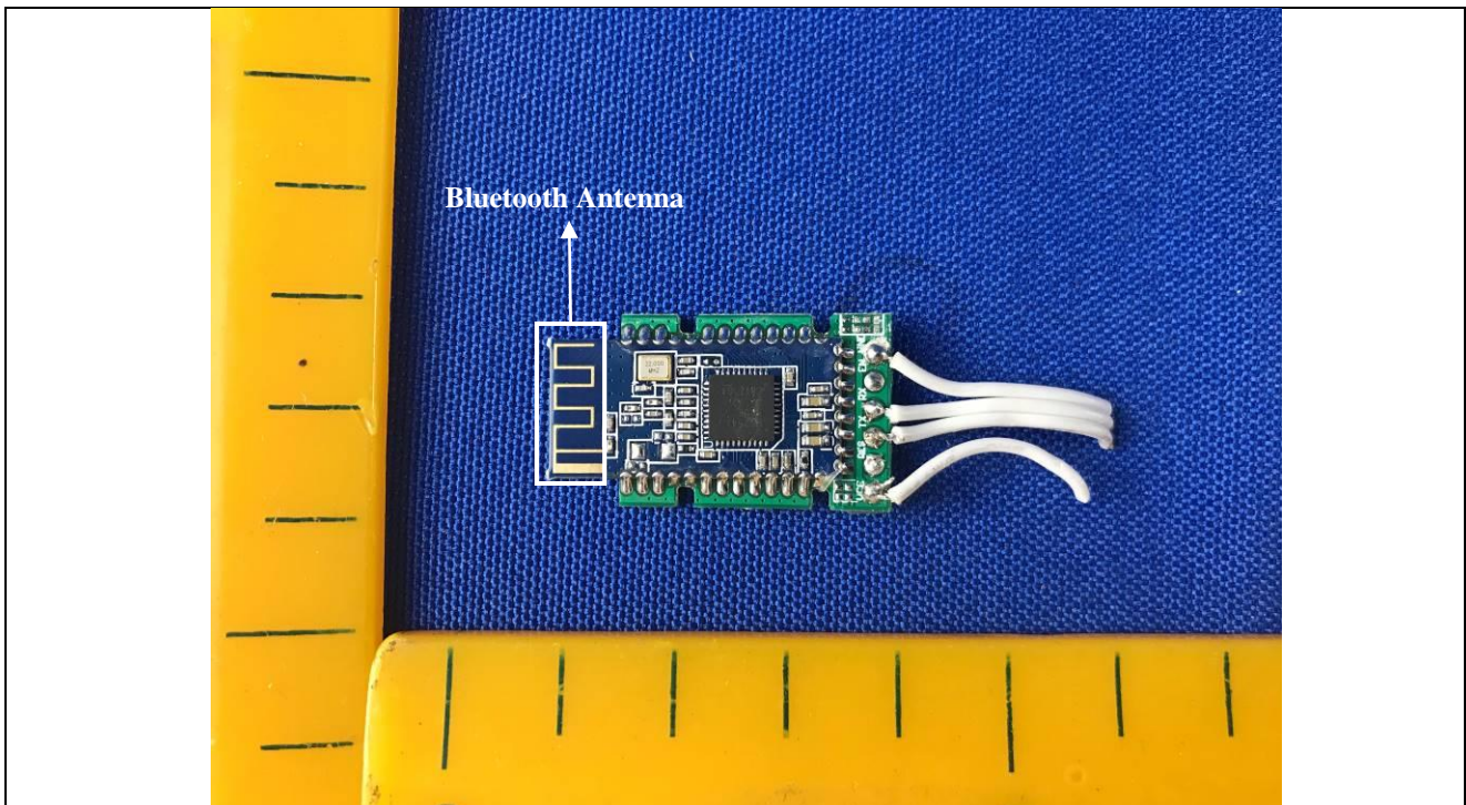
Details of: PCB view for Bluetooth module
