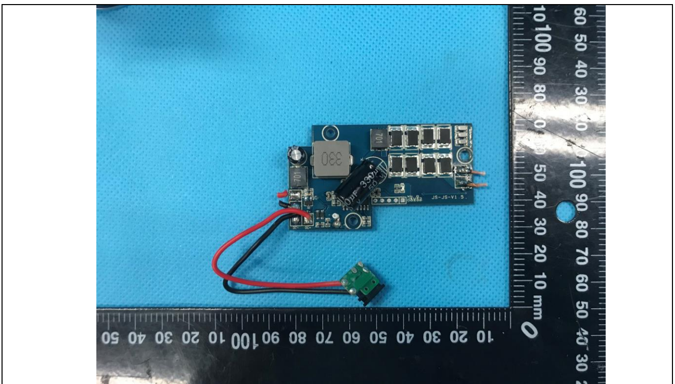
Details of: Wireless charging receiver board
