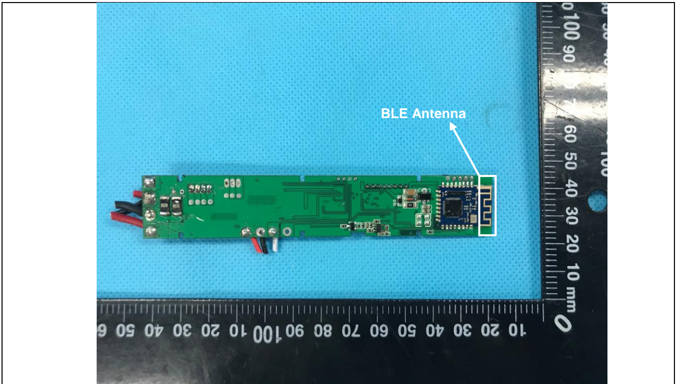
Details of: Main board
