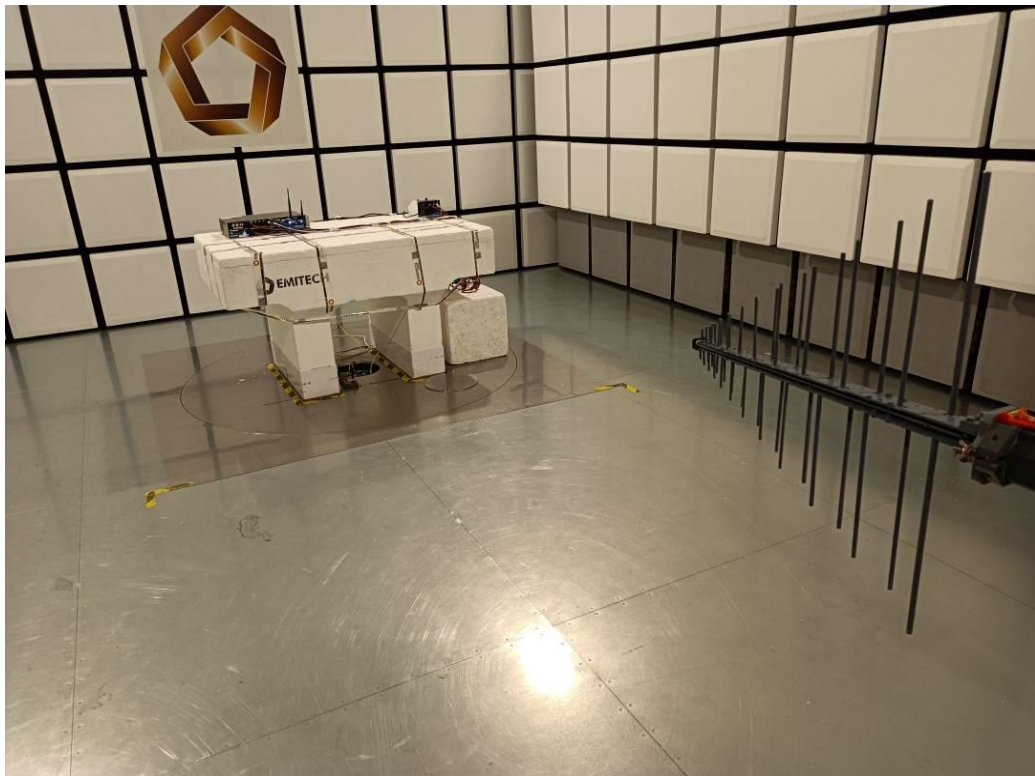
TEST SETUP PHOTO(S) - SETUP FOR 200MHZ < FREQ < 1GHZ
