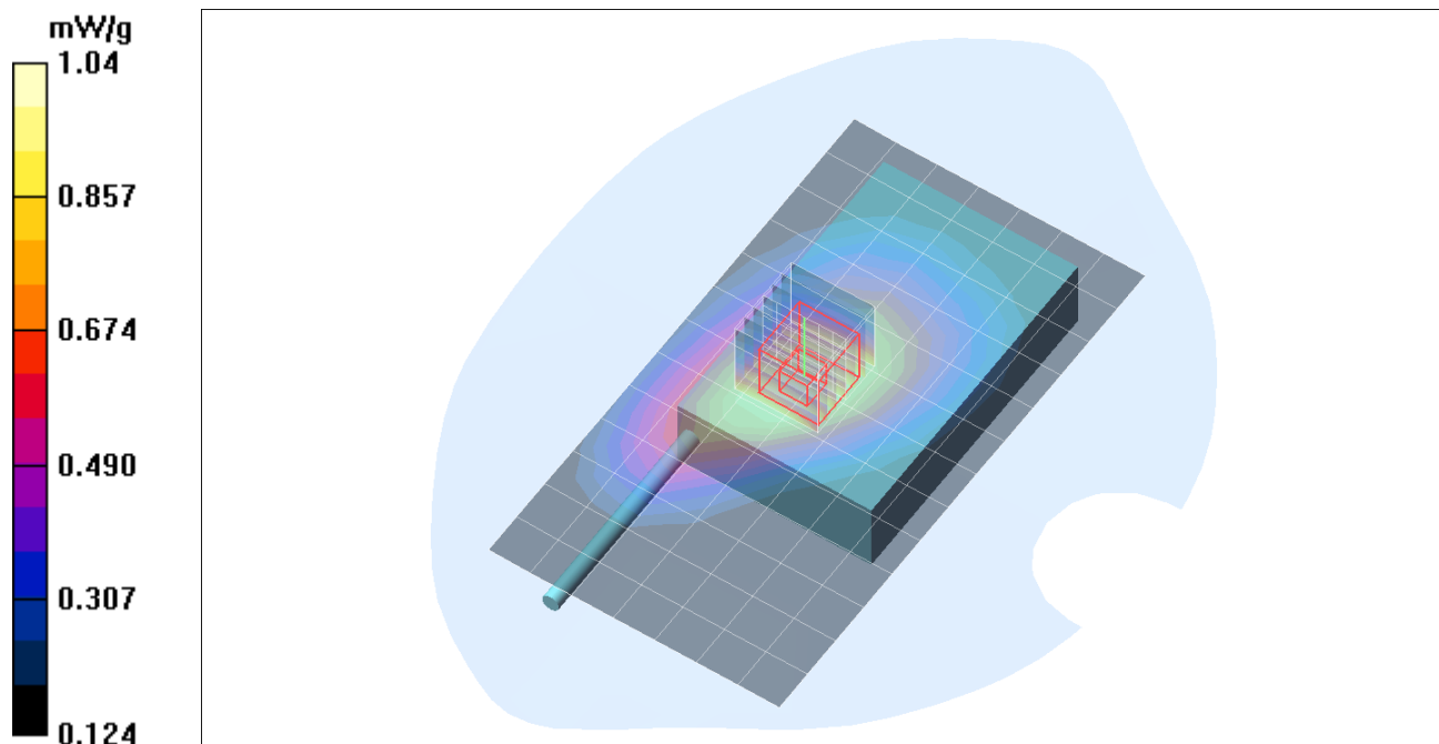
Plot. 1: SAR distribution plot for Guardian, low channel, back side of EUT toward the phantom, belt clip and headset attached.
