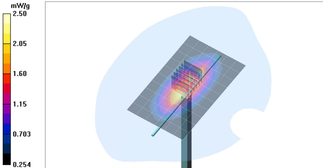
Plot. 2: System Verification Measurement 835 MHz, body.
