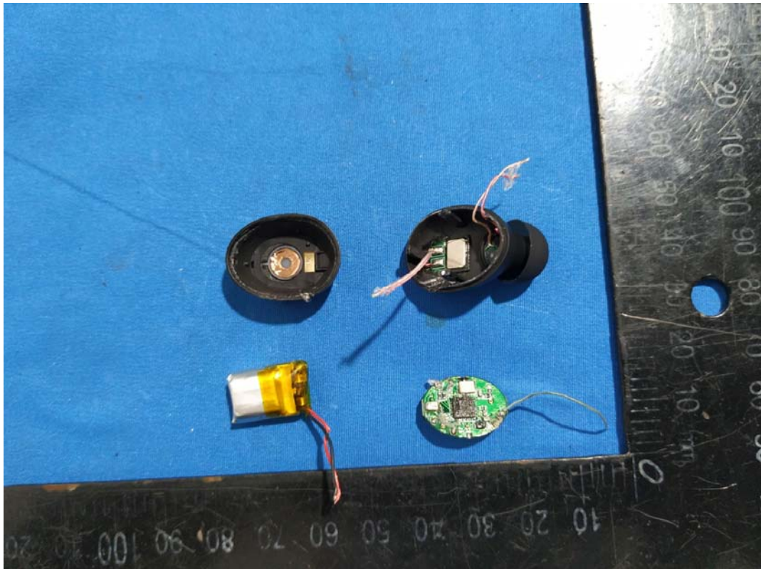
Right Earbuds
