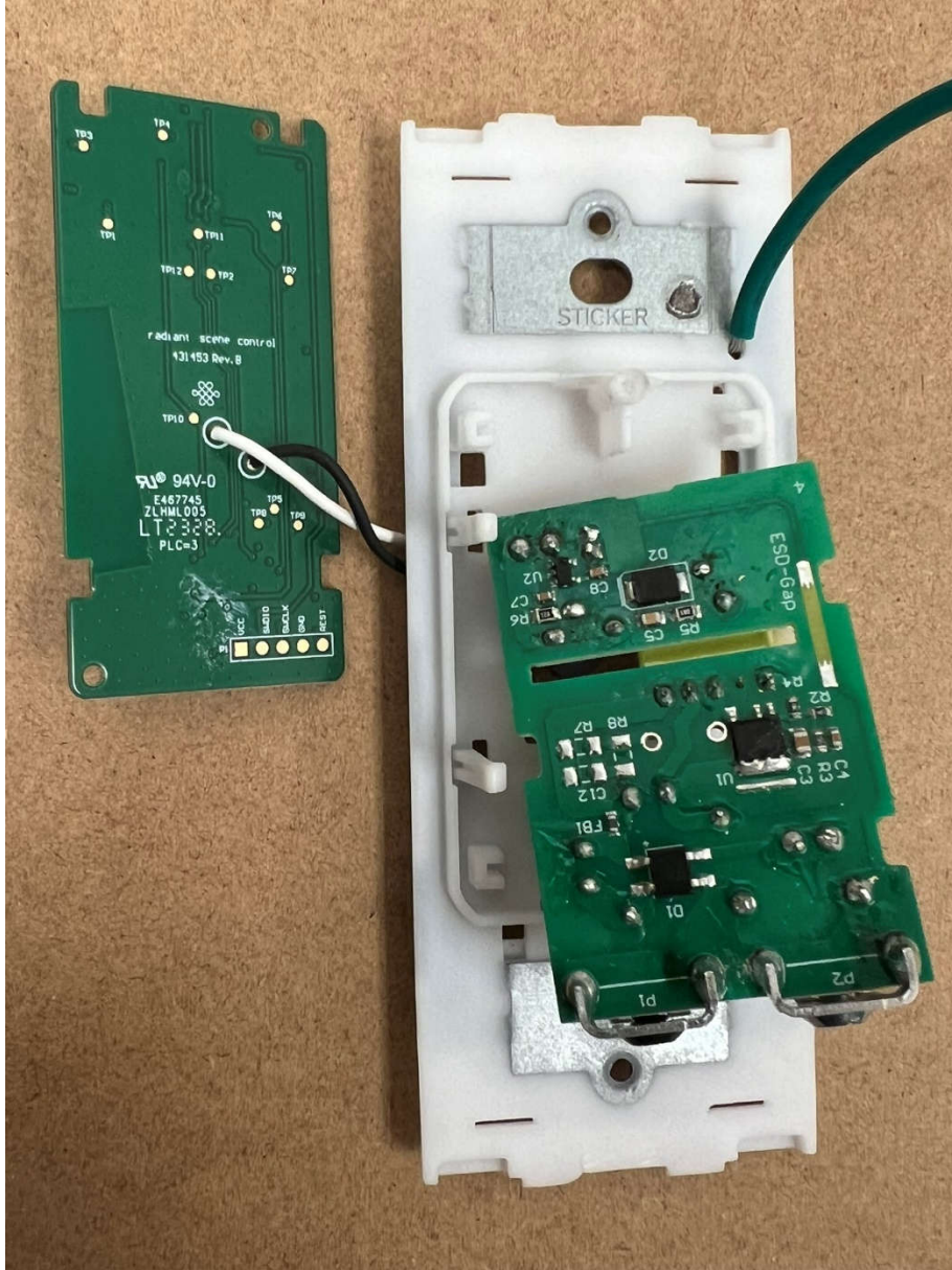
WZ3RCB46 RF Board Back Side (Left) – AC Board Top Side (Right)
