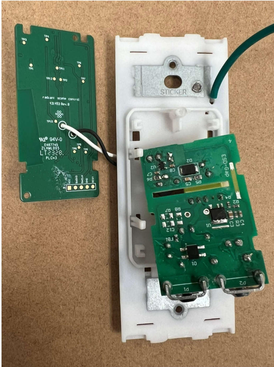
WNRCB46 RF Board Back Side (Left) – AC Board Top Side (Right)
