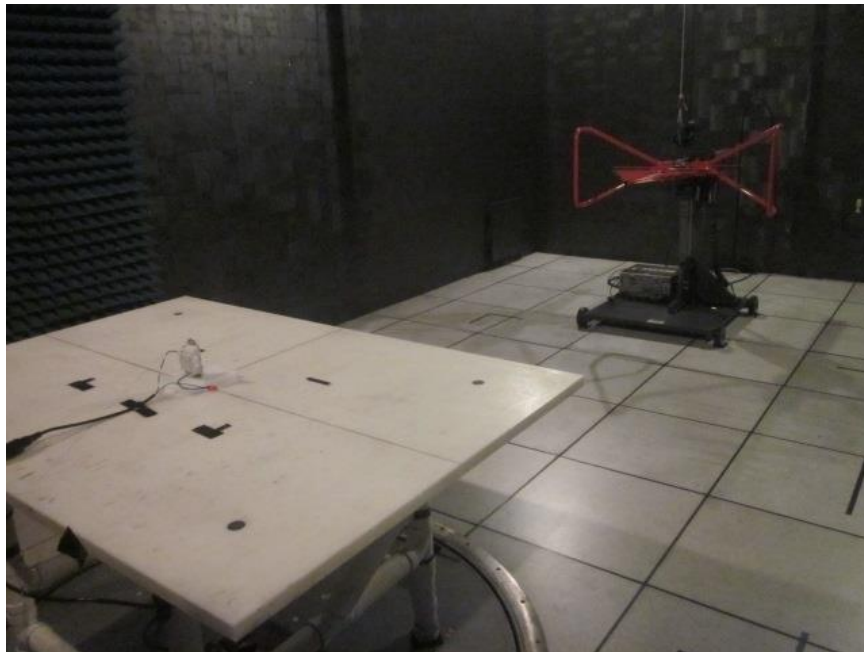
Radiated Emissions Test Setup 30 to 1000 MHz Shielded Room
