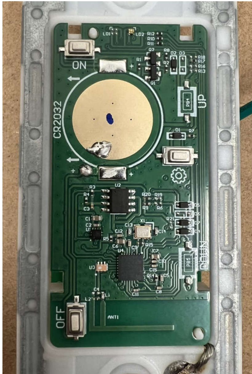
WZ3RL34 RF Board -Top
