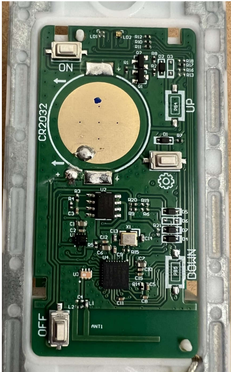
WZ3RL24 RF Board -Top
