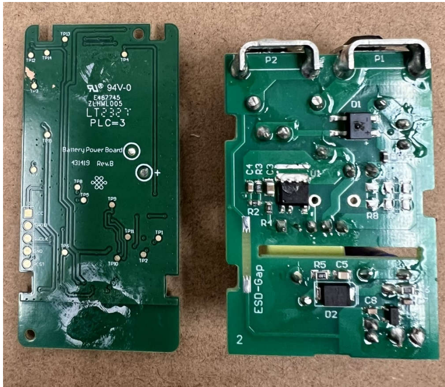
WNRL24 RF Board Back Side (Left) – AC Board Top Side (Right)
