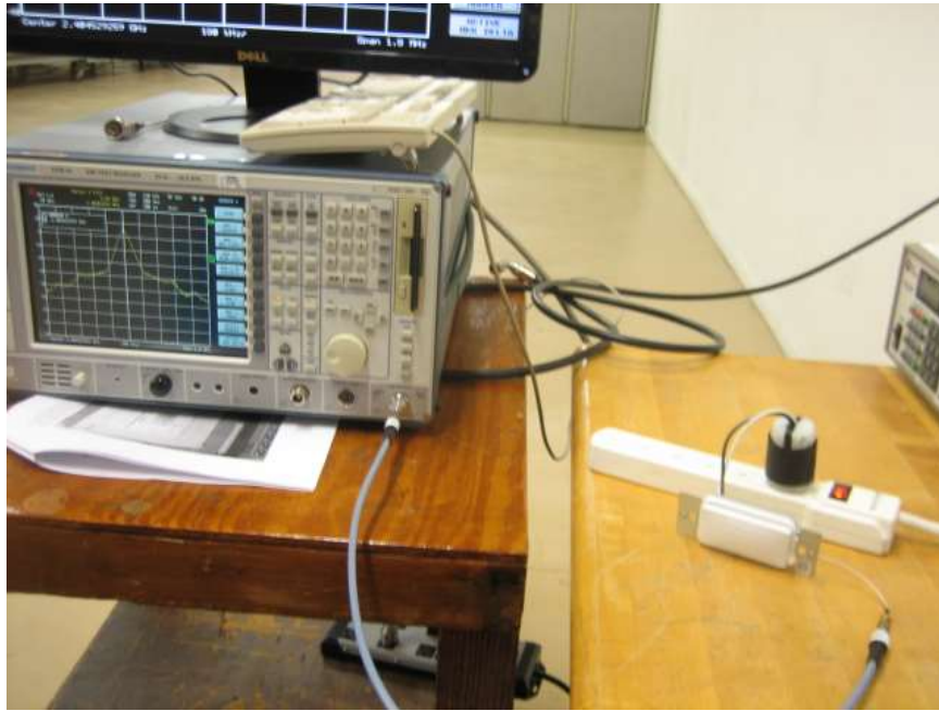
Antenna Conducted Test Setup
