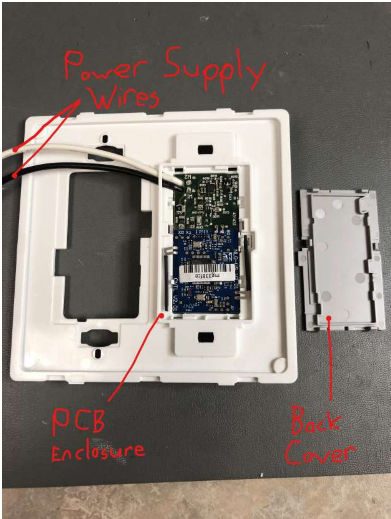
Figure 5: WNRH2 Assembly View
