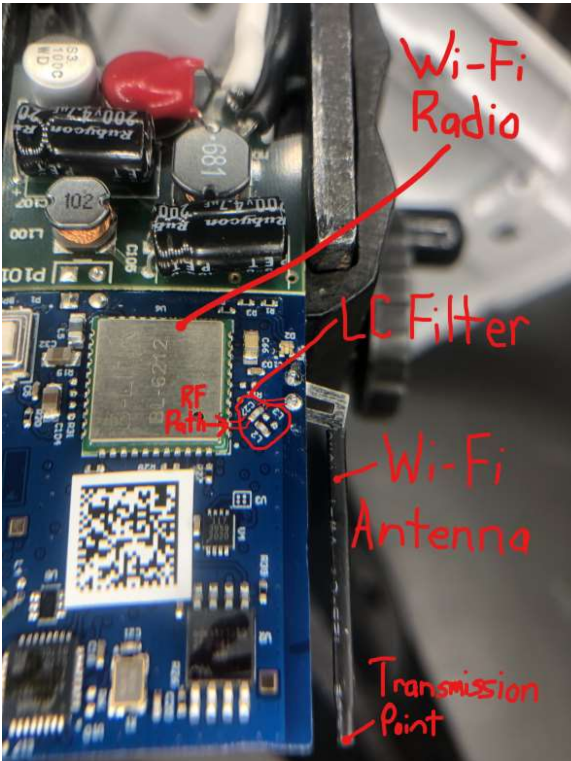
Figure 3: WNRH2 Wi-Fi Antenna
