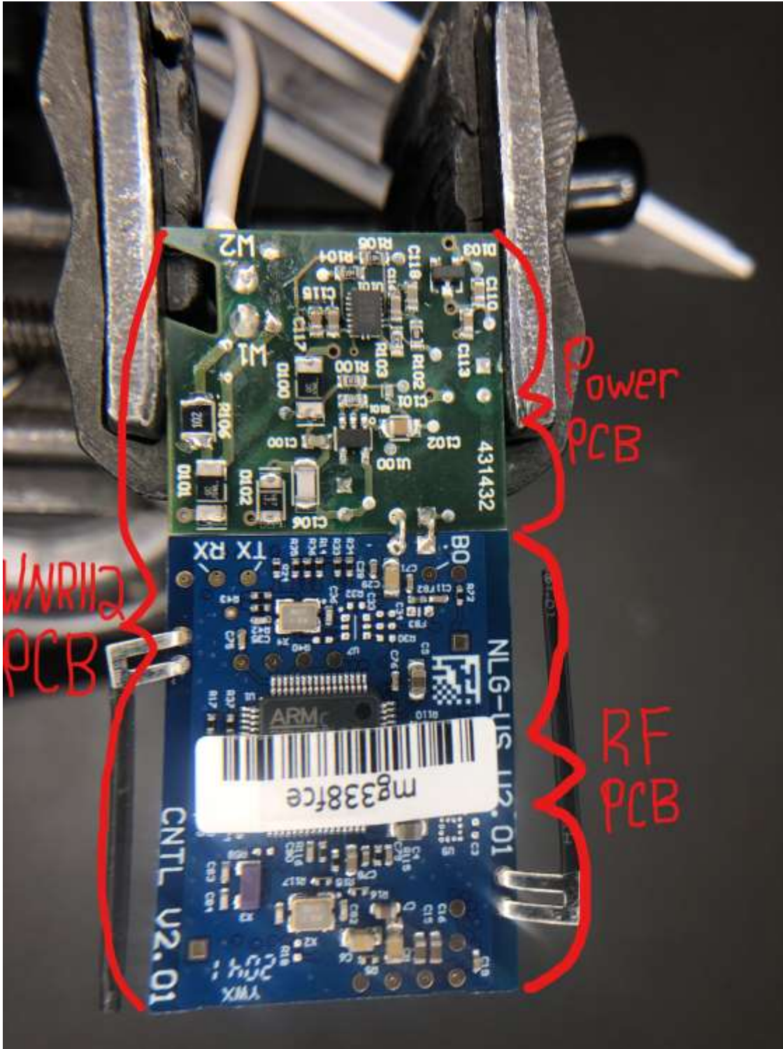
Figure 1: WNRH2 PCB Front View
