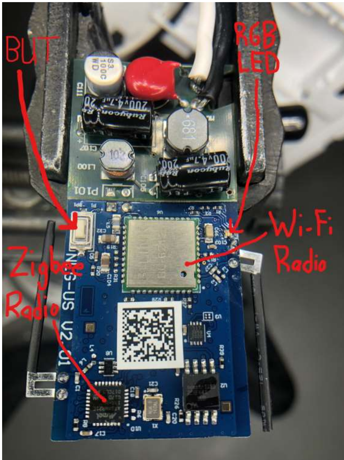
Figure 2: WNRH2 PCB Rear View
