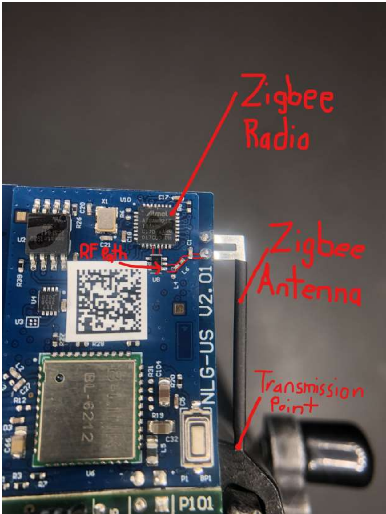
Figure 4: WNRH2 Zigbee Antenna
