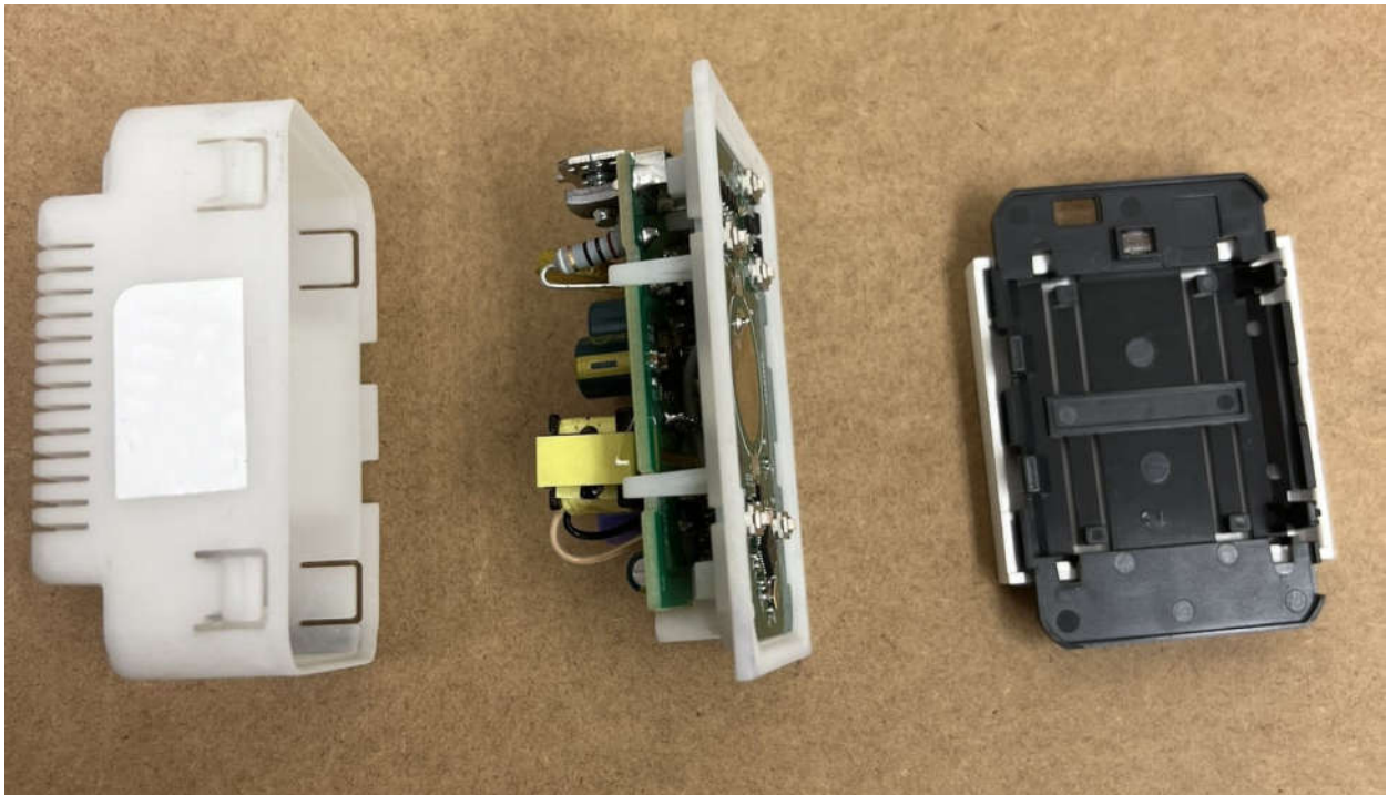
WZ3ABC46 Front and Back Cover Removed
