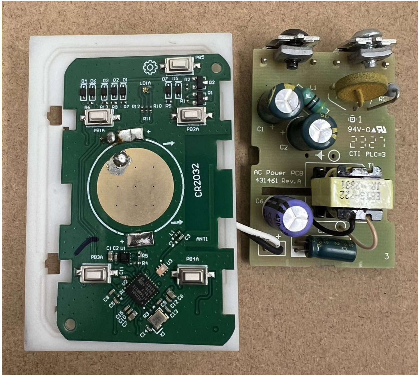
WZ3ACB46 RF Board -Top (Left), AC Board Bottom (Right)
