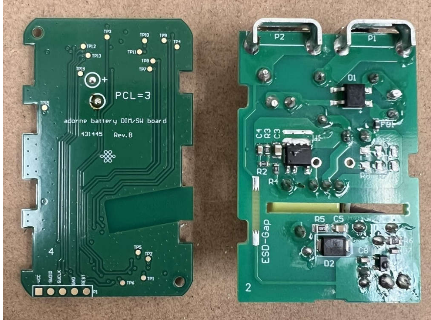
WZ3AL64 RF Board Back Side (Left) – AC Board Top Side (Right)
