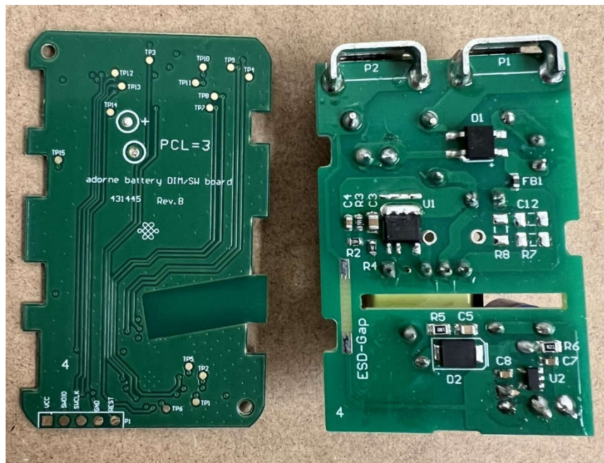
WZ3AL24 RF Board Back Side (Left) – AC Board Top Side (Right)
