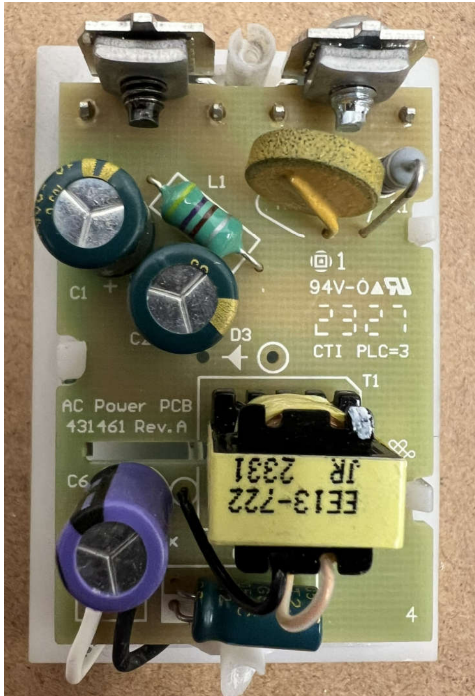
WZ3AL24 AC Board Back Side
