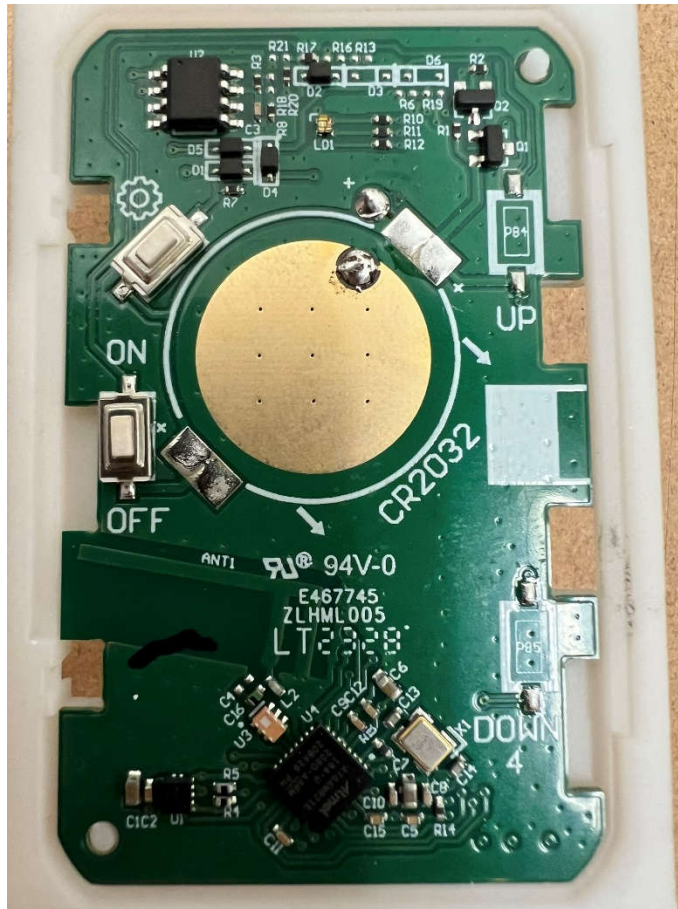
WZ3AL24 RF Board -Top
