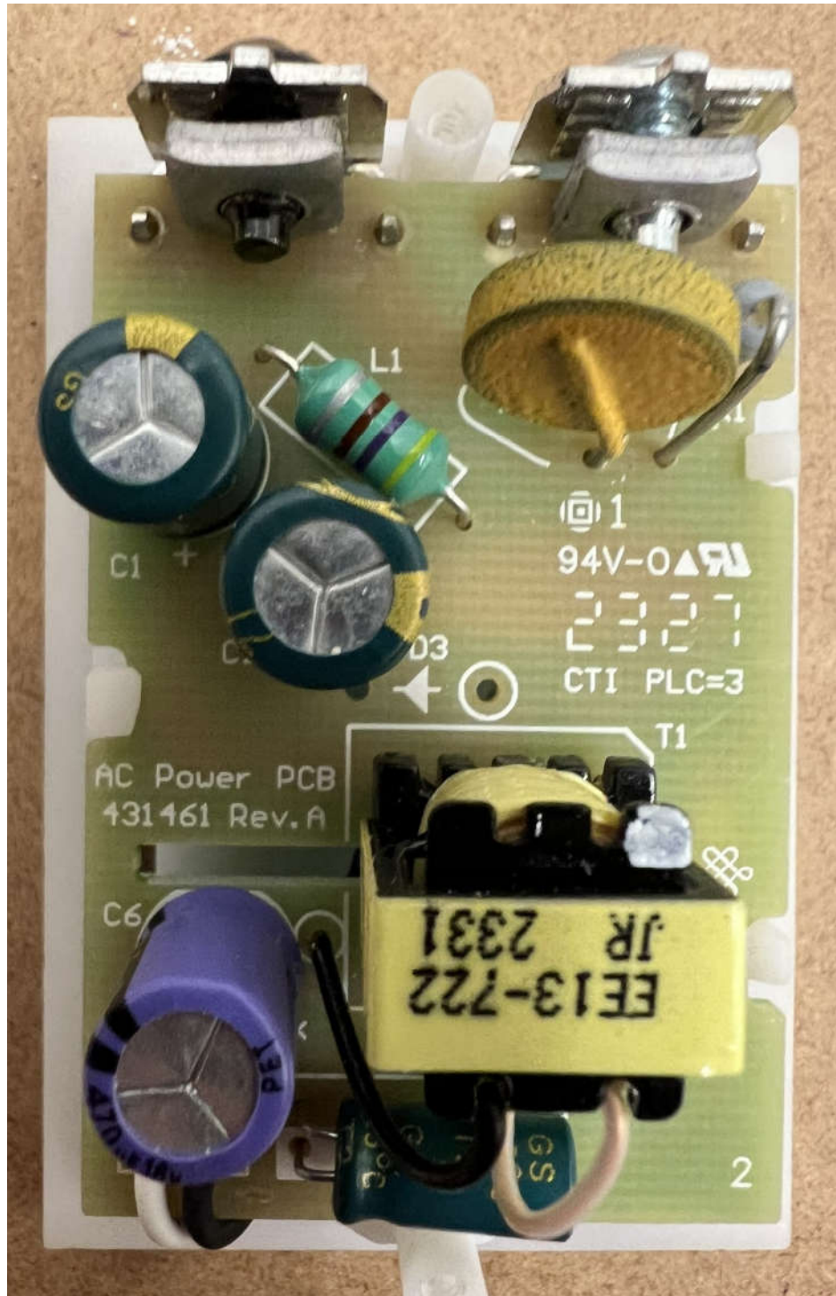
WZ3AL44 AC Board Back Side
