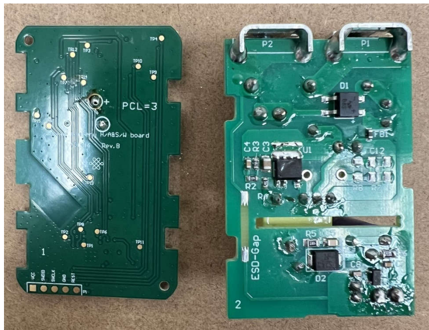
WZ3AL44 RF Board Back Side (Left) – AC Board Top Side (Right)
