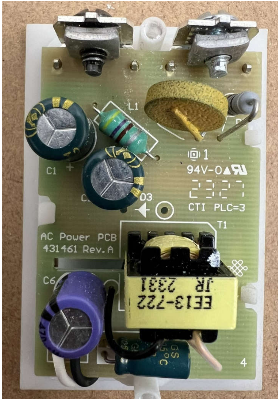
WZ3AL34 AC Board Back Side
