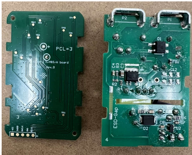
WNAL34 RF Board Back Side (Left) – AC Board Top Side (Right)
