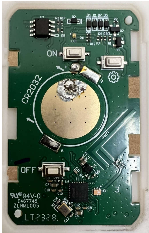
WNAL34 RF Board -Top
