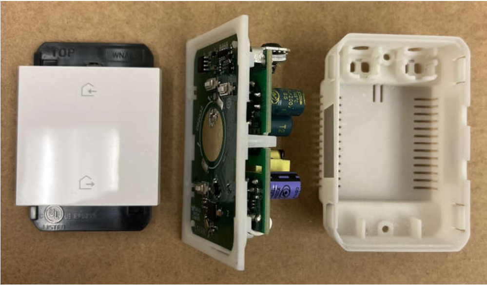
WNAL34 Front and Back Cover Removed
