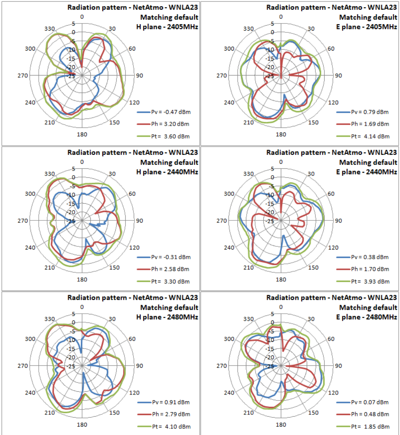
figure 16. From left to right, from top to bottom, Radiation pattern for H & E planes for the 2405, 2440 & 2480MHz frequencies for WNAL23 with default matching network
