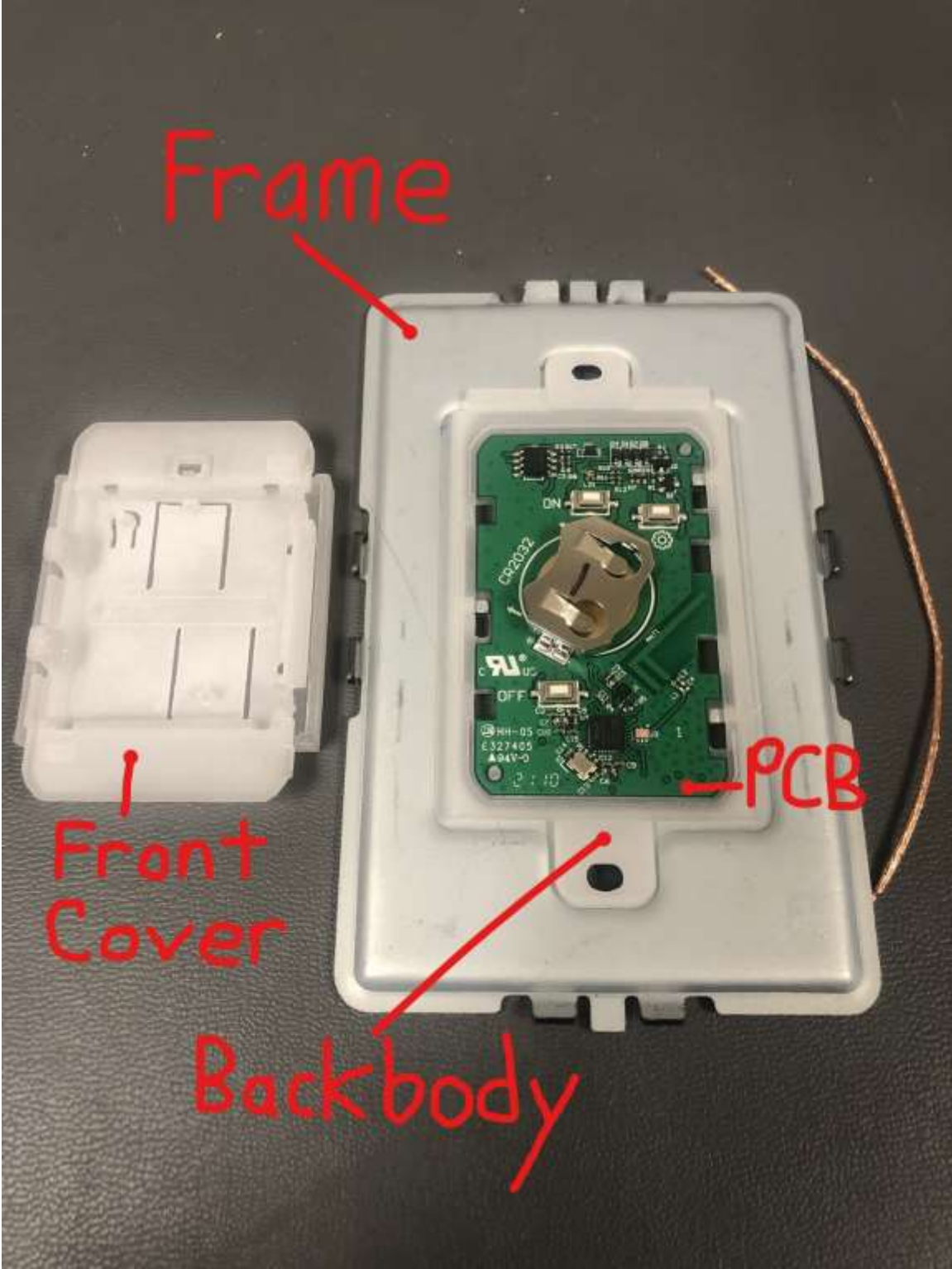
Internal Photo Legrand Model WNAL43 Assembly View
