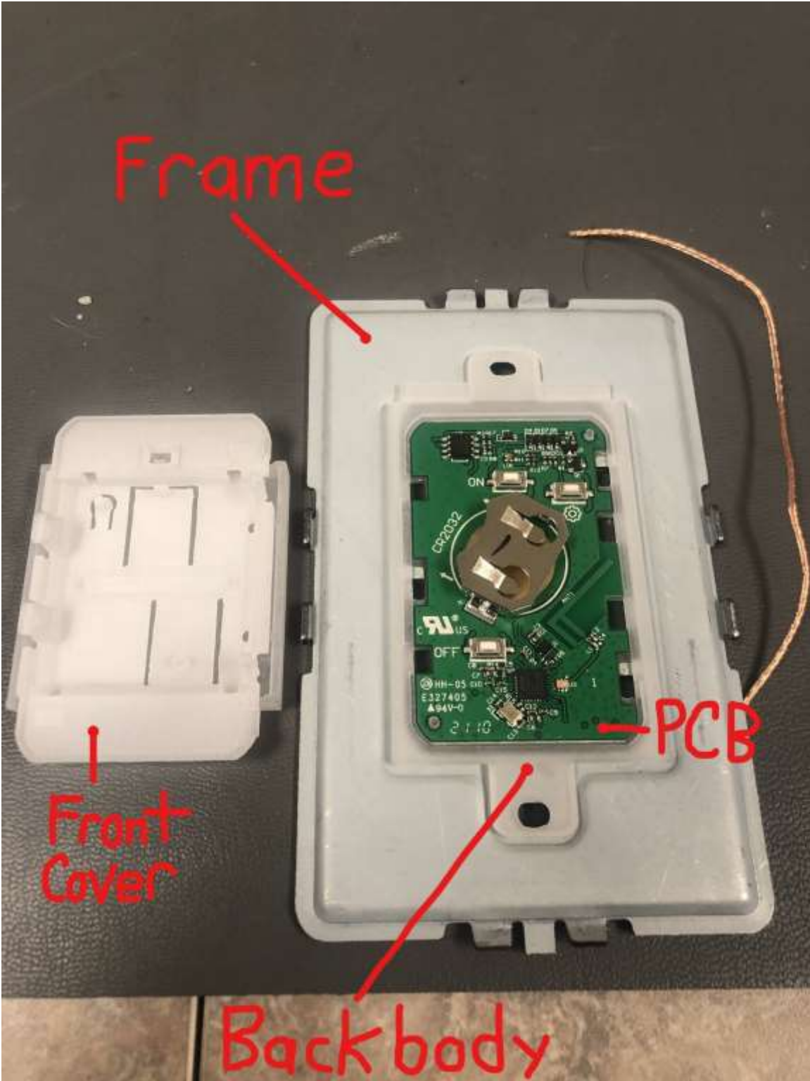
Internal Photo Legrand Model WNAL33 Assembly View
