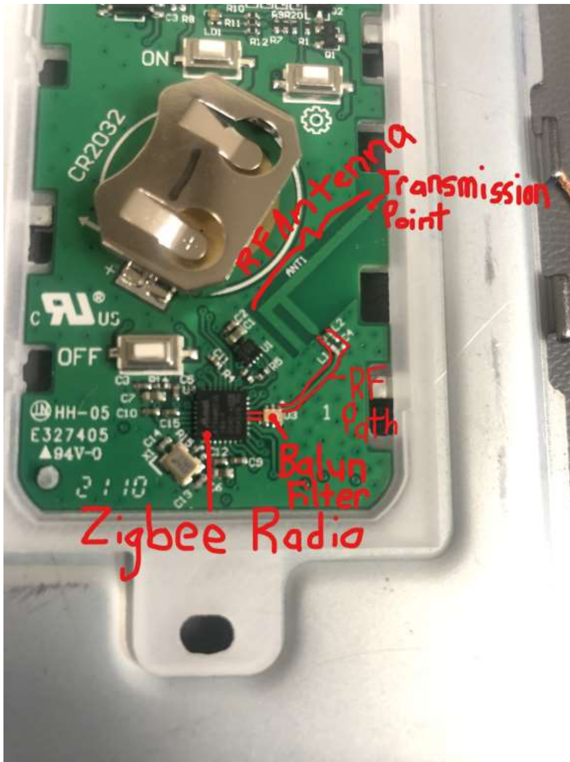
Internal Photo Legrand Model WNAL43 PCB View With Zigbee Radio Antenna Location
