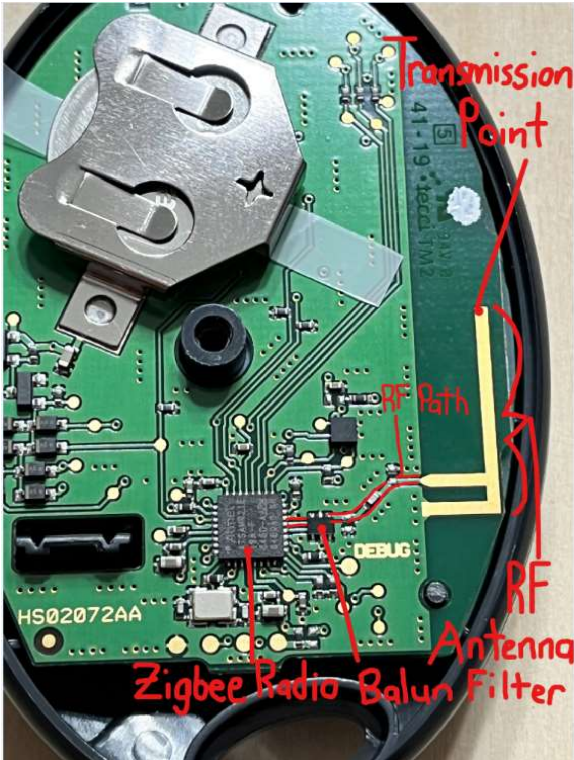
Zigbee Antenna View
