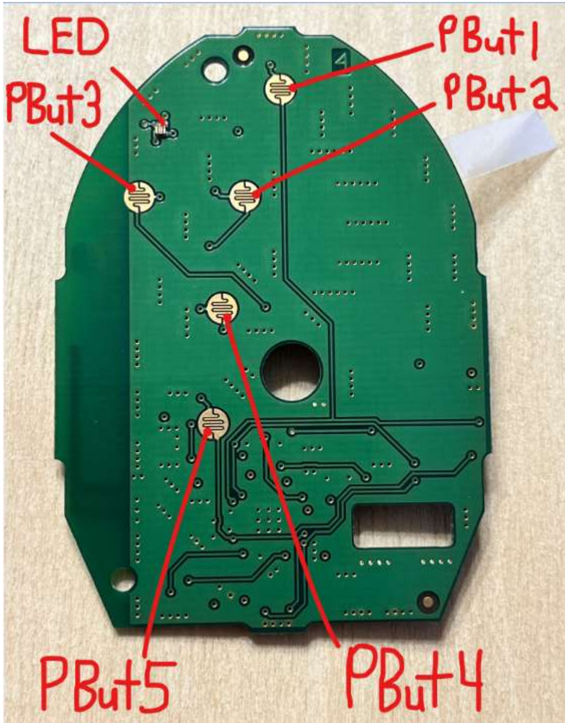
PCB Bottom View
