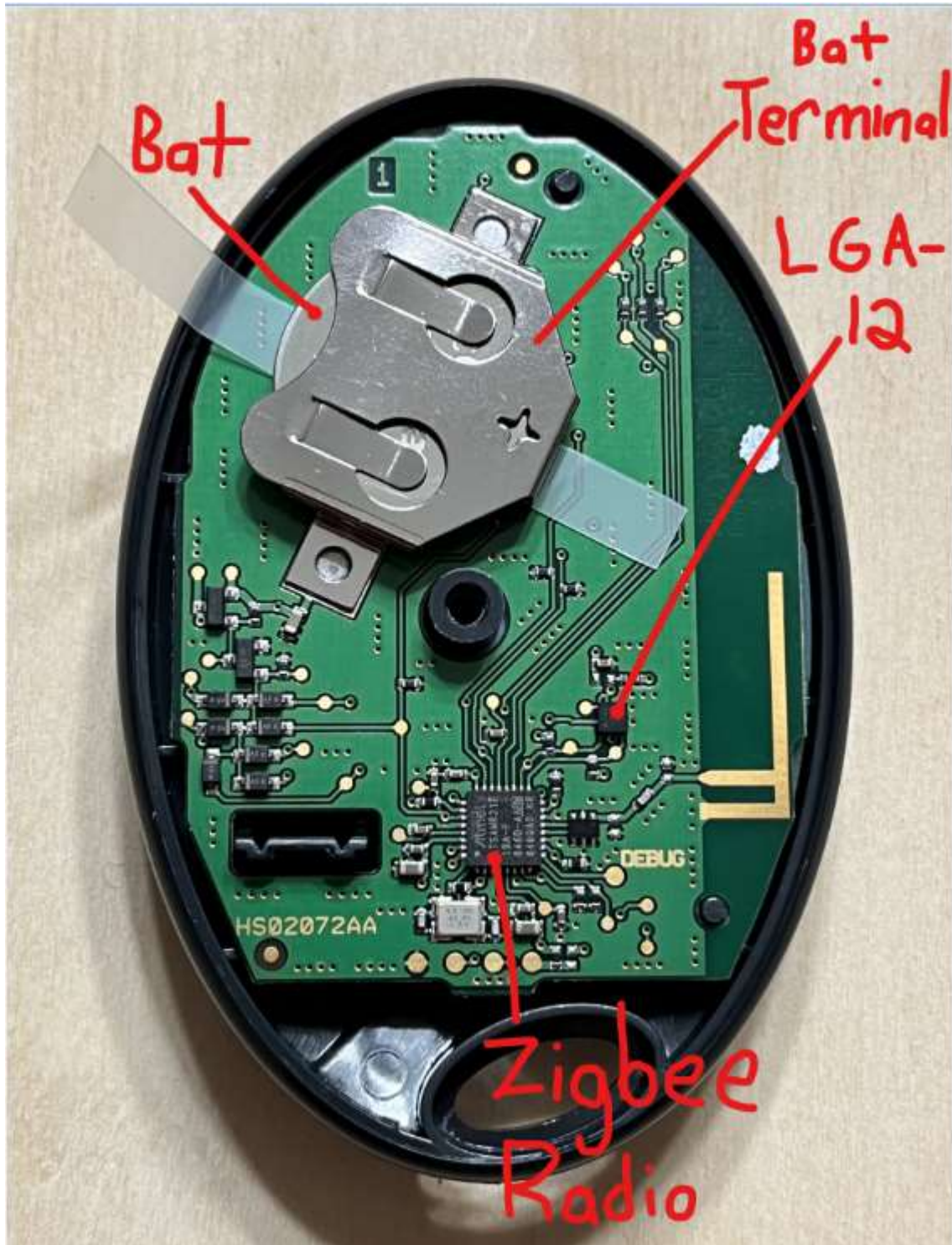
PCB Top View
