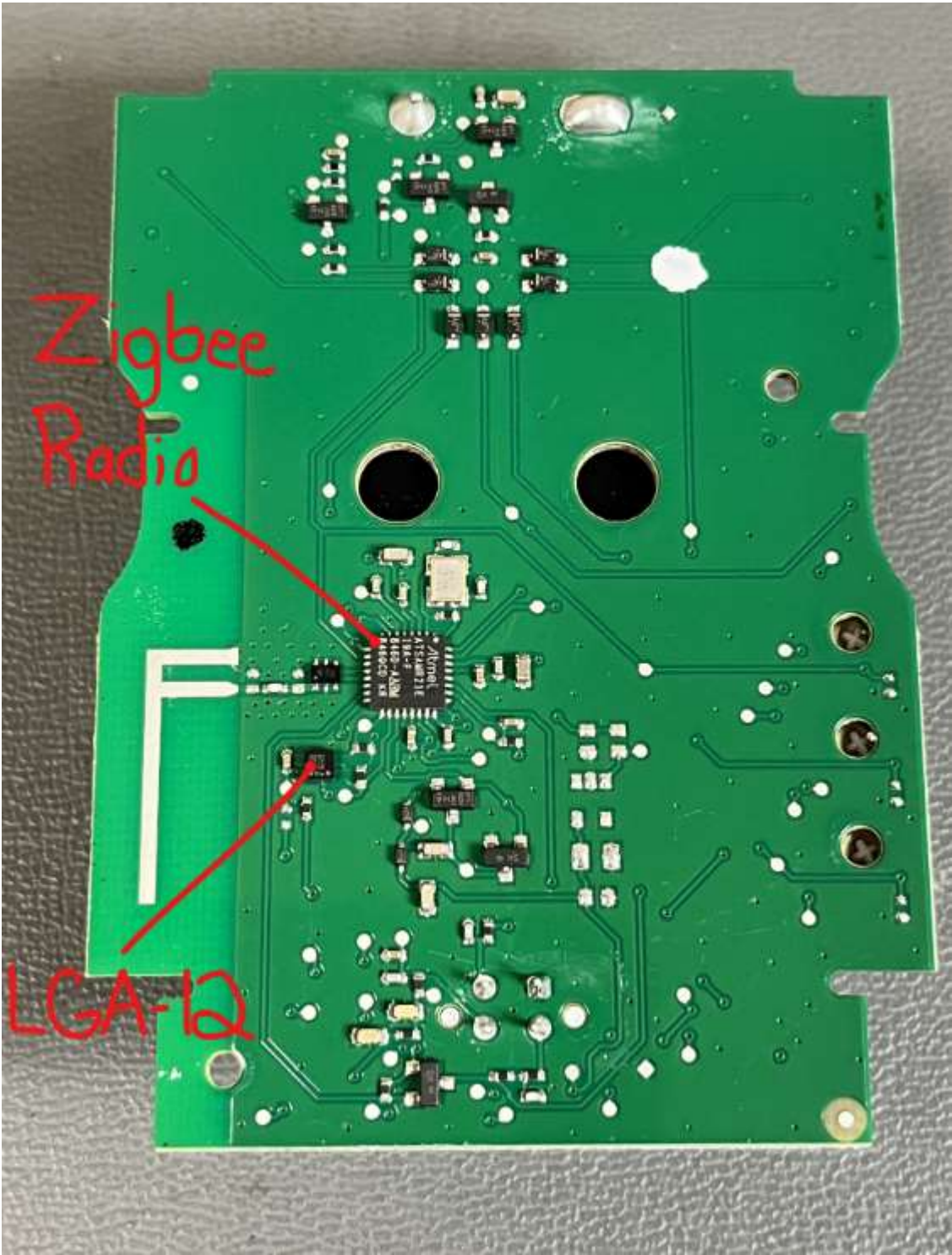
LEGRAND MODEL 064875 PCB BOTTOM VIEW
