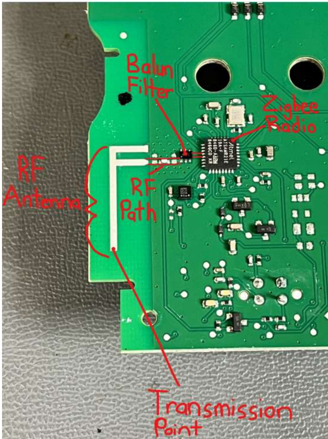
LEGRAND MODEL 064875 ZIGBEE ANTENNA VIEW
