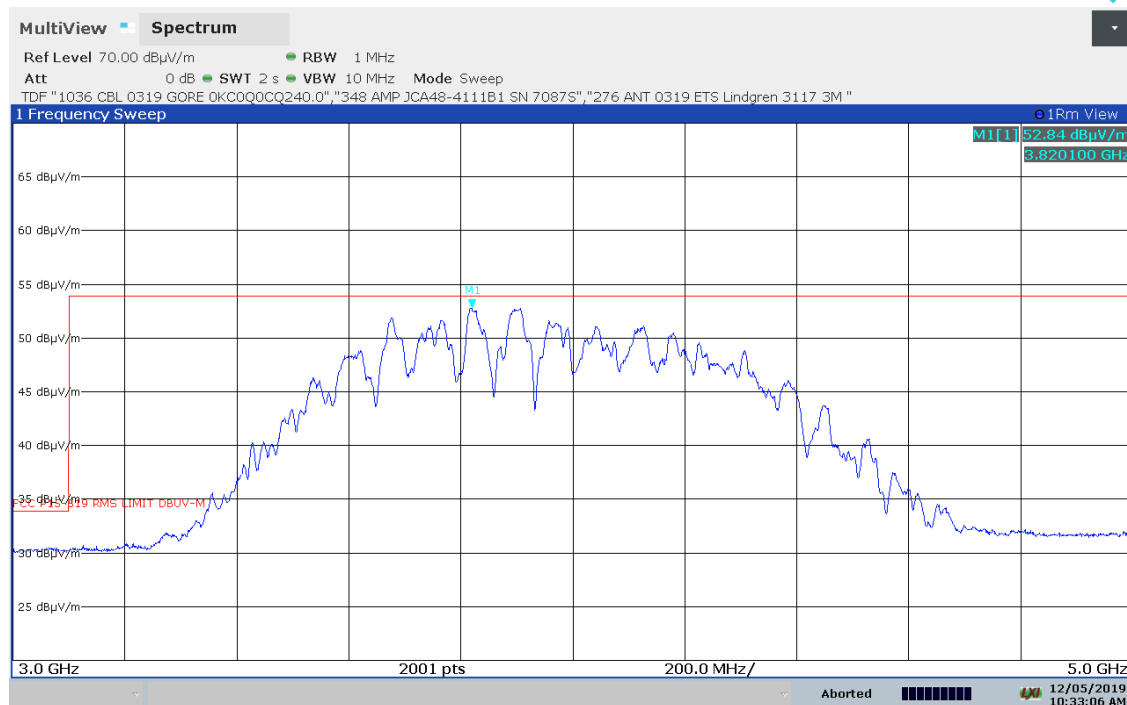
458-19 Racelogic Beacon
