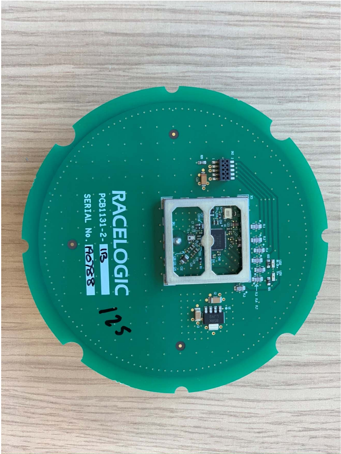
RF board component side – no shield
