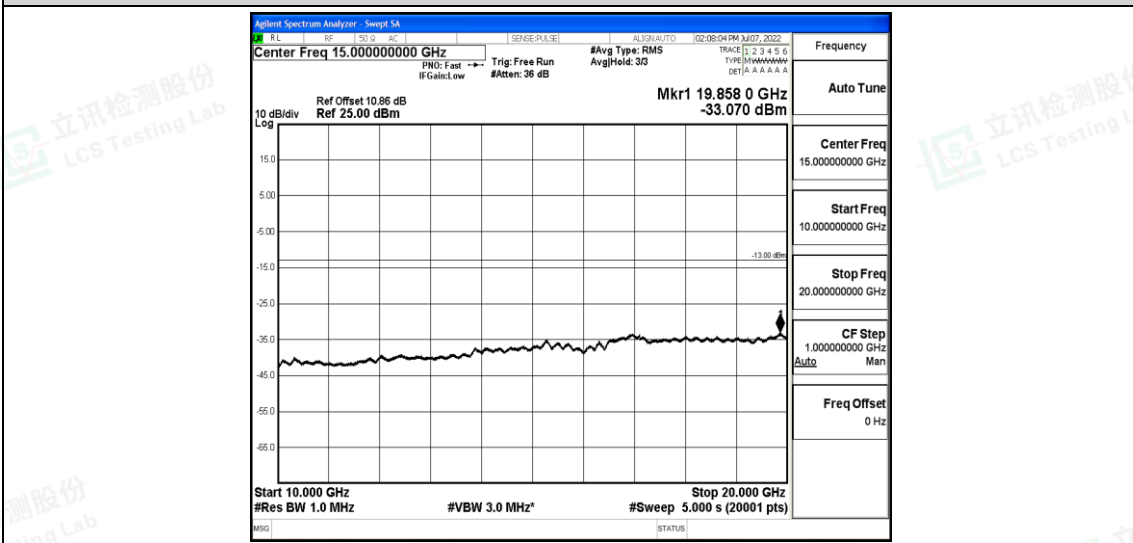
Band4-20MHz-16QAM-20300-1RB#0-Range5:10000~20000MHz
