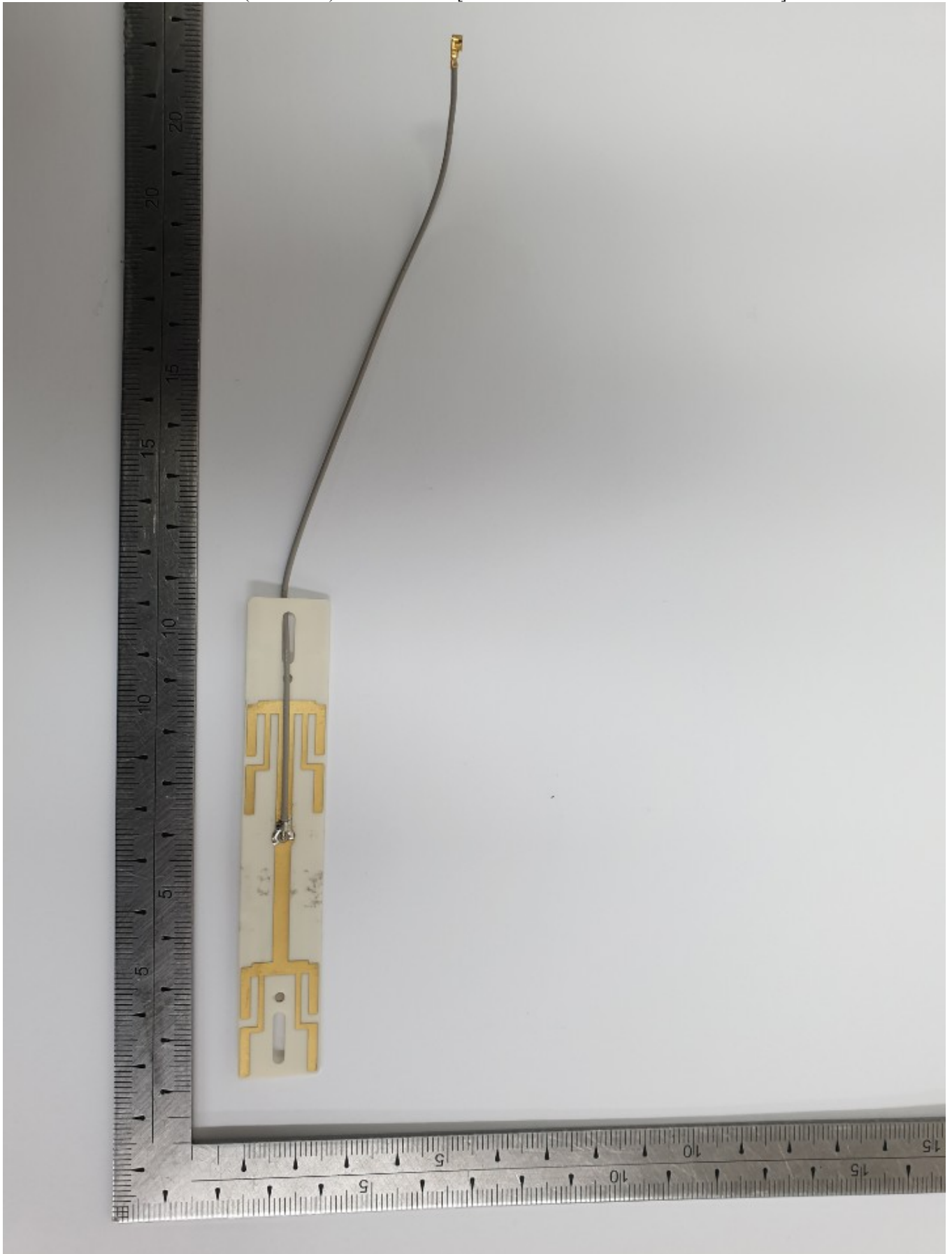
Antenna 4 (Additional) / PCB Antenna [Model name: AEi-RO-5500DP4-IPEX160]
