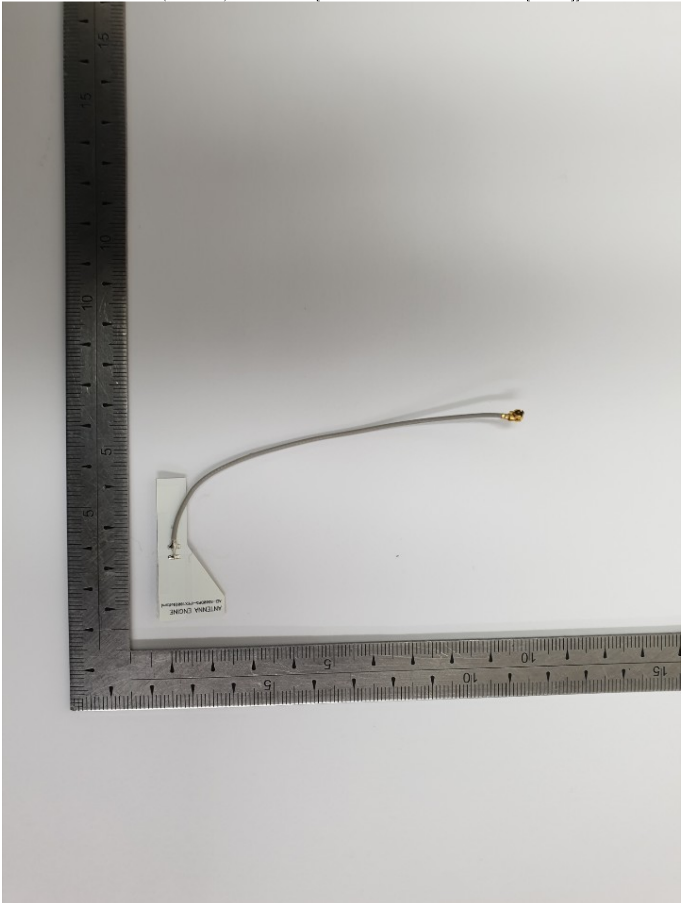
Antenna 3 (Additional) / PCB Antenna [Model name: AEi-5500DP5-IPEX100[Bottom]]
