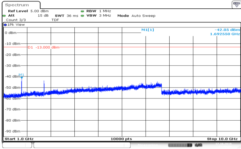
Band5-5MHz-QPSK-20625-25RB#0-Range4:1000~10000MHz
