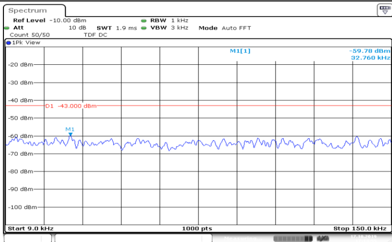
Band5-10MHz-16QAM-20450-50RB#0-Range1:0.009~0.15MHz
