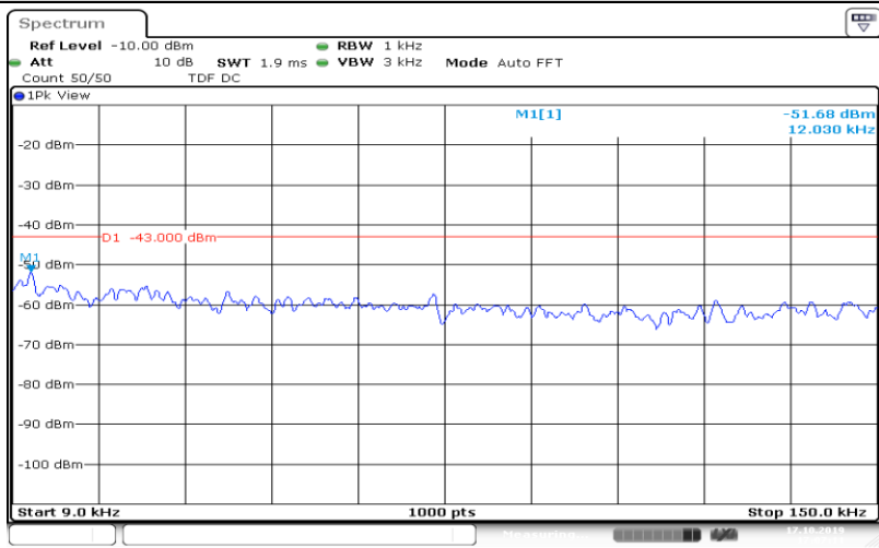
Band5-5MHz-16QAM-20425-25RB#0-Range1:0.009~0.15MHz
