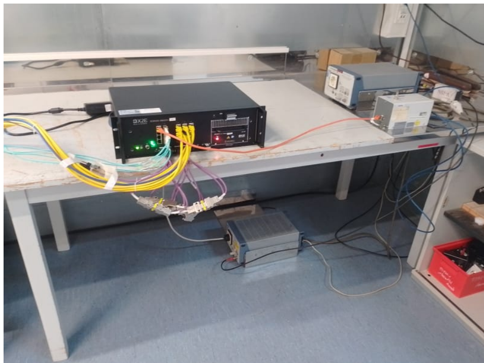
Photo 1: conducted emission
