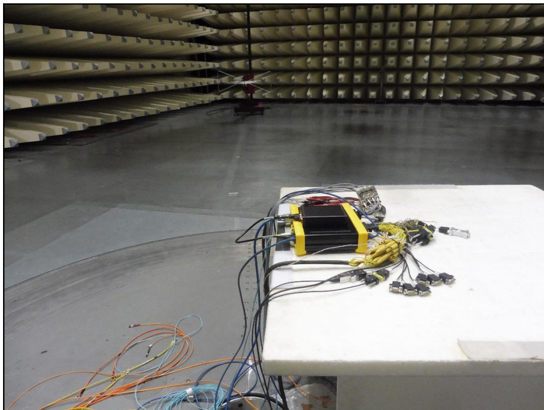
Photo 5: radiated emission
