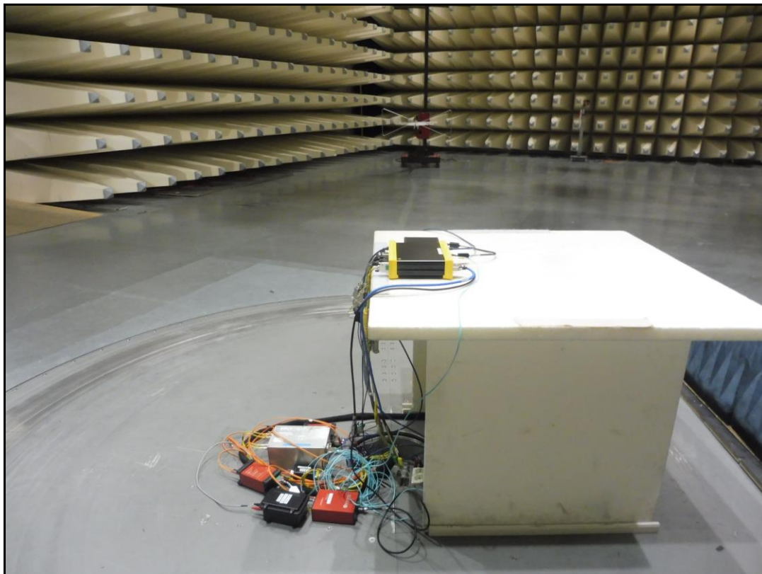
Photo 3: radiated emission
