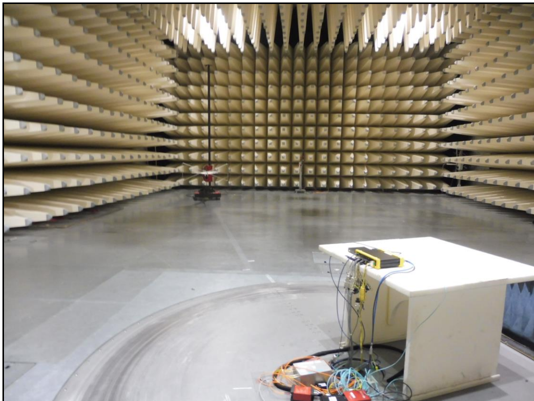
Photo 2: radiated emission
