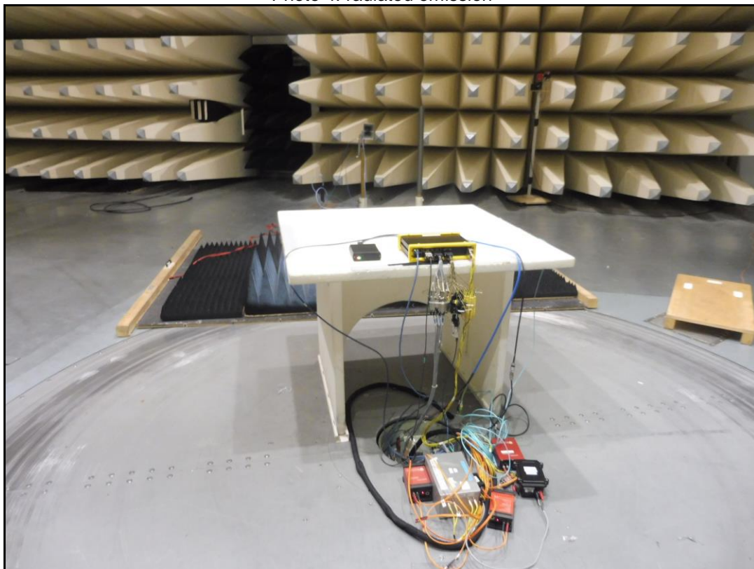
Photo 4: radiated emission
