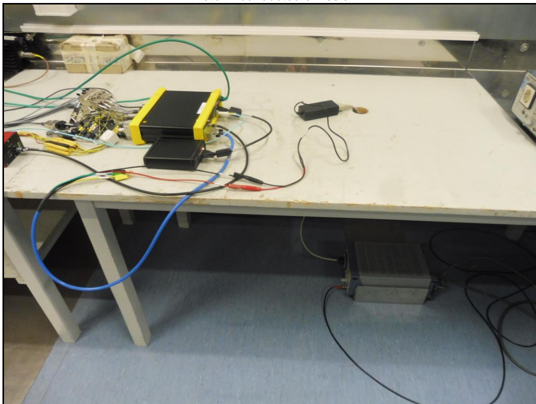
Photo 1: conducted emission
