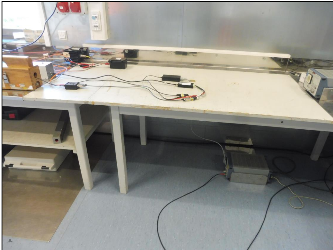
Photo 3: conducted emission
