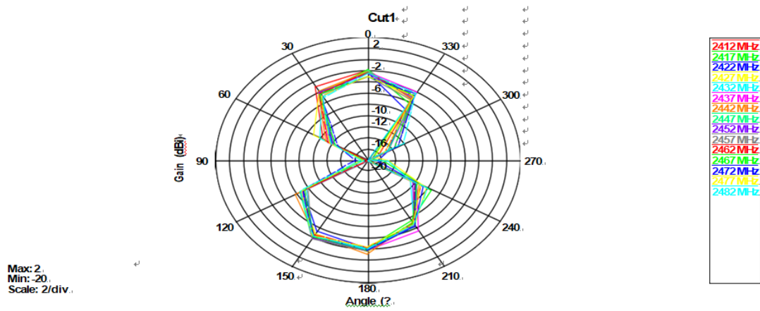
Vertical Y-Z
