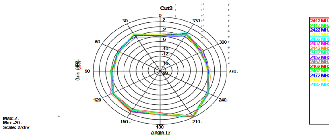
Vertical X-Z
