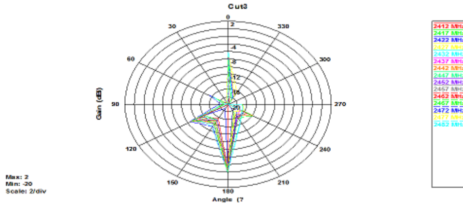
Vertical X-Y
