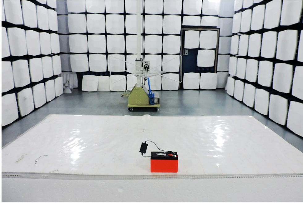
Radiated Emission Test Setup:
