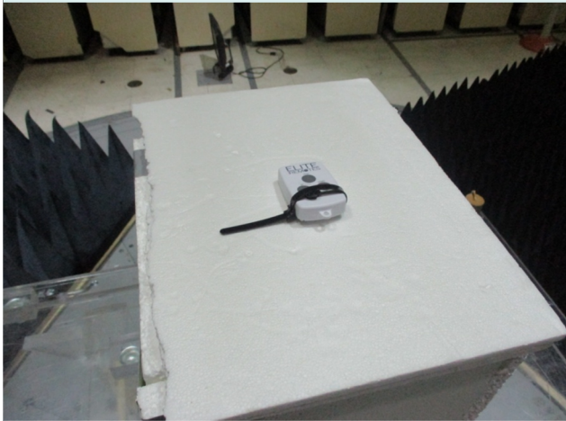
EUT Setup Position (worst case)
