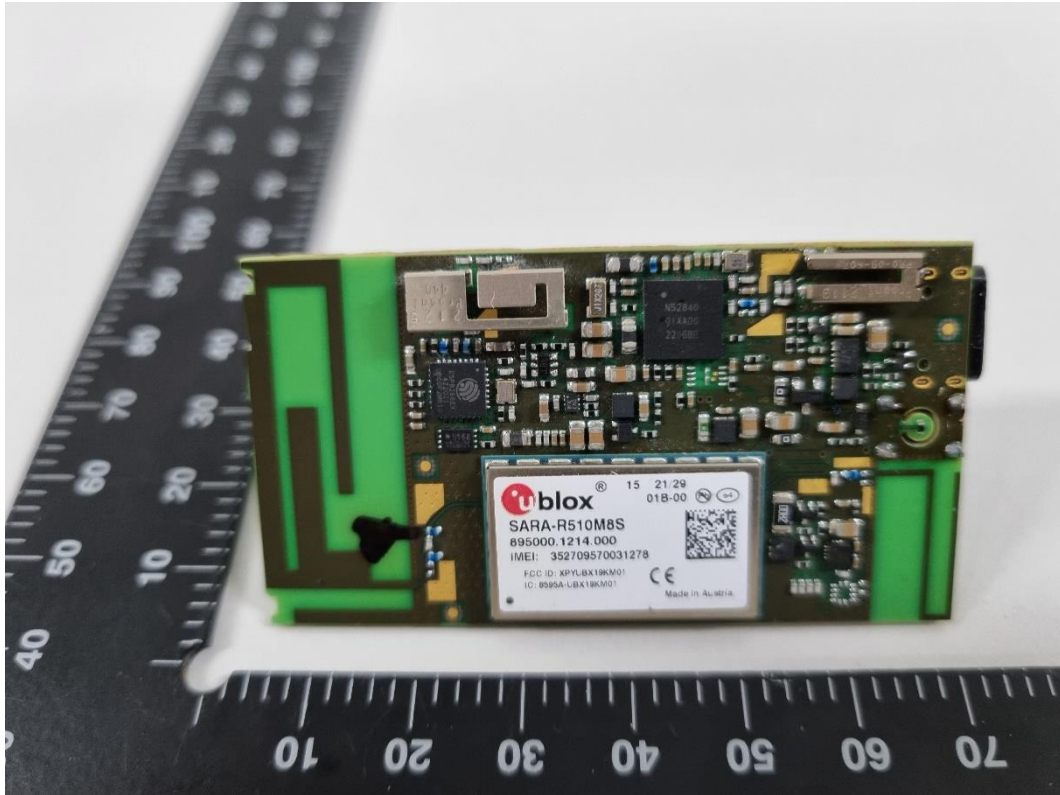
Main Board(front)
