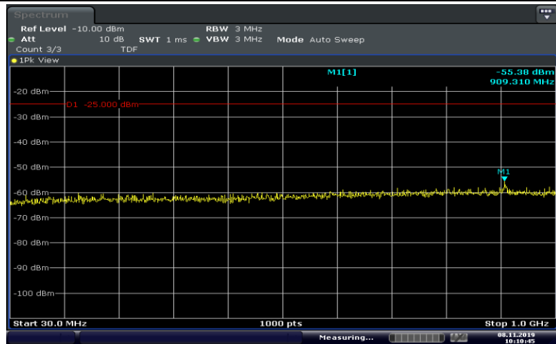
Band41-5MHz-QPSK-40265-25RB#0-Range1:30~1000MHz
