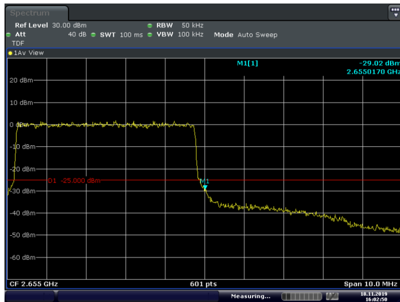
Band41-5MHz-QPSK-41215-25RB#0
