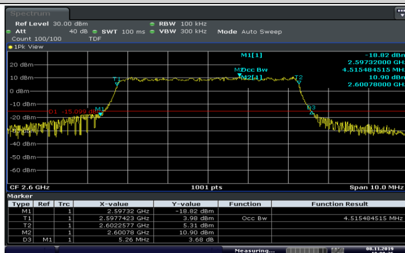
Band41-5MHz-QPSK-40690-25RB#0-4.515
