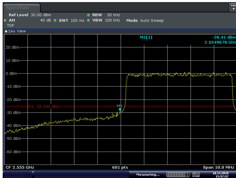
Band41-5MHz-QPSK-40265-25RB#0
