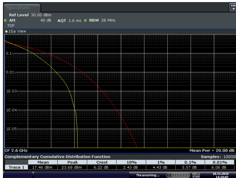
Band41-5MHz-QPSK-40690-25RB#0
