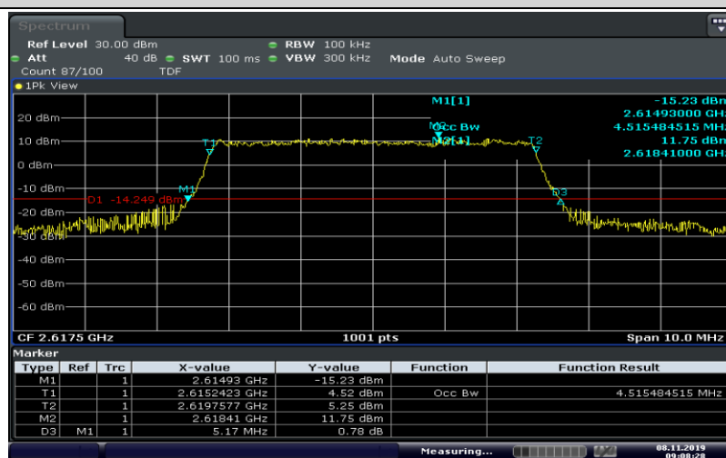
Band38-5MHz-QPSK-38225-25RB#0-4.515
