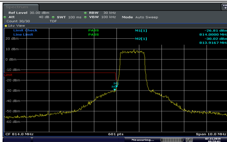
Band26-1.4MHz-16QAM-26697-6RB#0
