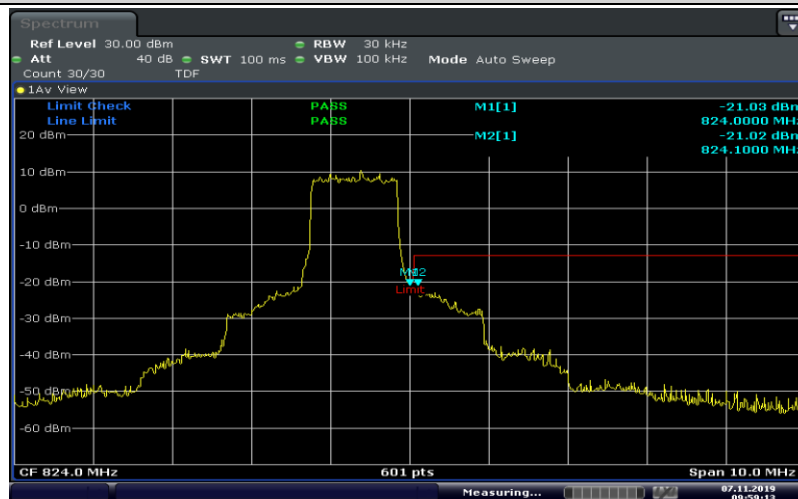
Band26-1.4MHz-QPSK-26783-6RB#0
