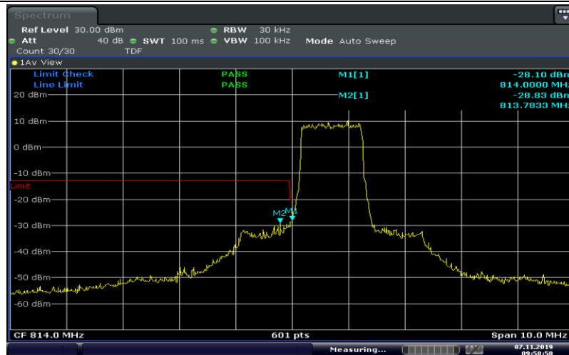
Band26-1.4MHz-QPSK-26697-6RB#0
