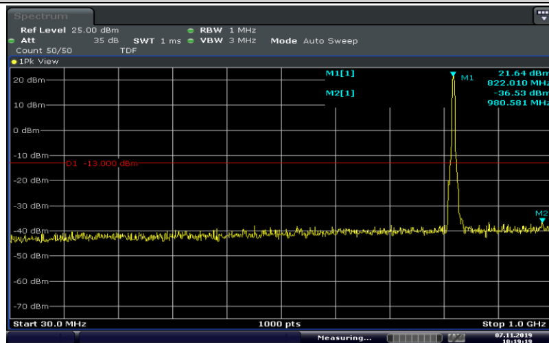
Band26-5MHz-16QAM-26765-25RB#0-Range3:30~1000MHz
