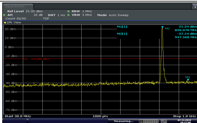
Band26-5MHz-QPSK-26740-25RB#0-Range3:30~1000MHz
