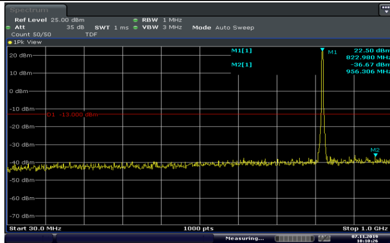
Band26-3MHz-QPSK-26775-15RB#0-Range3:30~1000MHz
