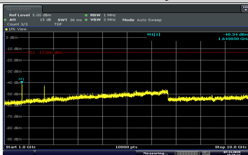
Band26-5MHz-16QAM-26765-25RB#0-Range4:1000~10000MHz
